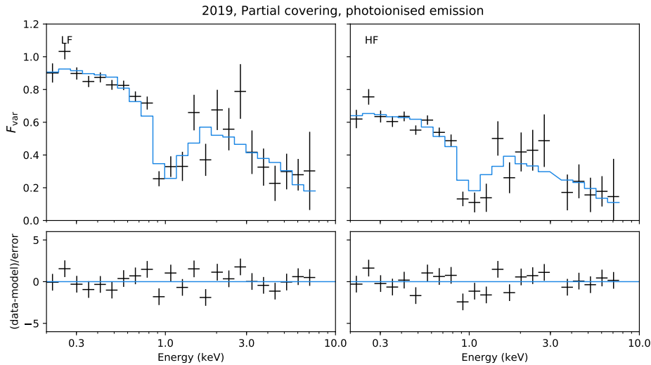
Figure 8. Photoionisation damped absorption fit to the 2019 F_{\text{var}} spectra, fit with the model \text{FVAR\_PION} \times \text{FVAR\_PCOV} . This fit gives a good description of the data, and the absorption interpretation explains the qualitative differences in the shape of the variance spectrum between the 2019 observation and the other epochs. Additional plots showing the fits with the intrinsic variability model and absorption without photoionised emission are presented in Fig. A3
