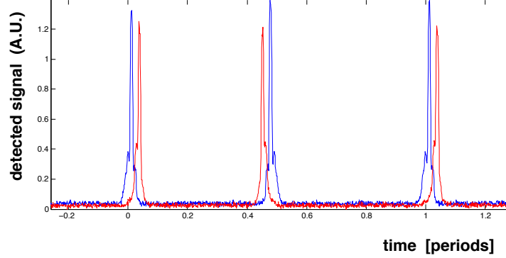
Figure 5: Each sensor (blue or red) detects the passage of the pendulum and a pulse is recorded. The order of pulse arrival depends on the sense of oscillation, but the pulse separation in time is the same
