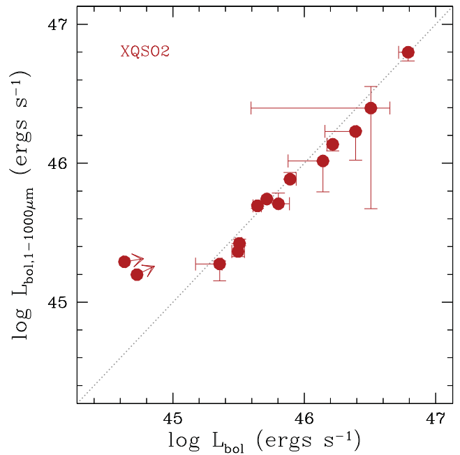
Figure 7. IR-based L_{bol} derived for the XQSO2s following the prescriptions by Pier & Krolik (1992) and Pozzi et al. (2007) versus the WISE-based L_{bol} derived by applying the relation between the WISE W3 data and the bolometric luminosity recovered from the analysis of the XQSO1s in the XBS; the bars identify the ranges of values obtained when all the possible modelling (with all the QSO templates and extinction curves) are considered. The arrows mark the two objects for which we are able to put only limits to the nuclear emission (namely, XBSJ052128.9–253032 and XBSJ080411.3+650906). The dotted line marks the one-to-one relation between the luminosities.
