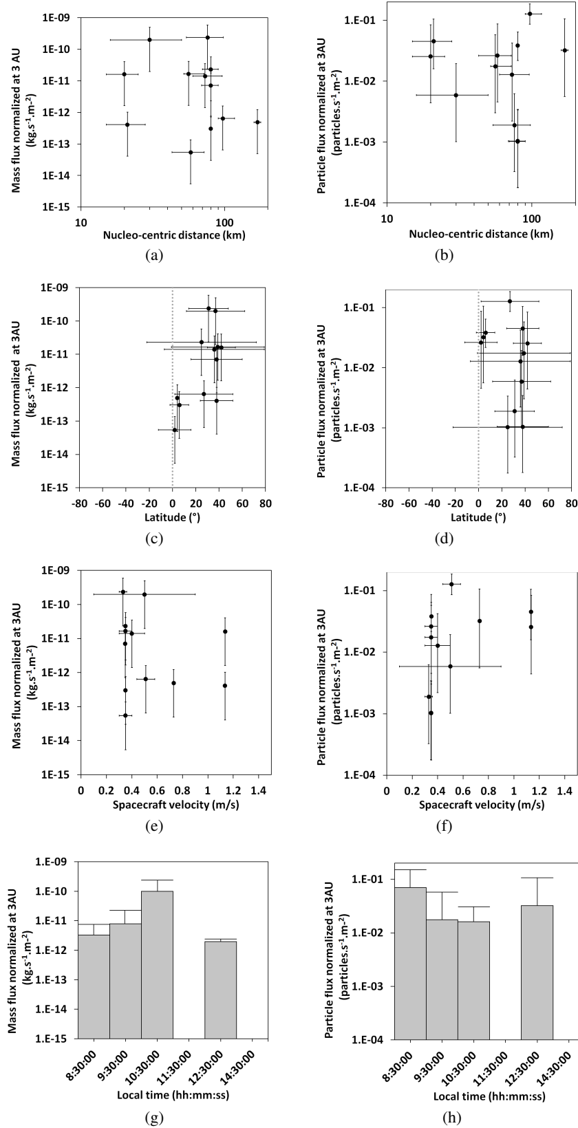
Fig. 5. Low phase angle ( 0^\circ – 45^\circ ) mass fluxes of dust ( left column ) and particle fluxes ( right column ) normalized to the solar distance at 3 AU and plotted against nucleo-centric distance a ), b ), latitude c ), and d ), spacecraft velocity e ), f ), and local time g ), h ). The error bars on the mass fluxes are given by using densities of 2500 \text{ kg/m}^3 and 100 \text{ kg/m}^3 . The error bars on the particle fluxes represent the 1\sigma error. For collection periods with low number of particles (less than 100), the error bars are derived from Gehrels (1986) .
