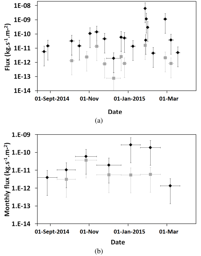
Fig. 9. Dust flux of porous aggregates (black diamonds) and compact particles (gray squares) larger than 100 \mu\text{m} a) , as well as their monthly average b) , from mid August 2014 to April 2015.
