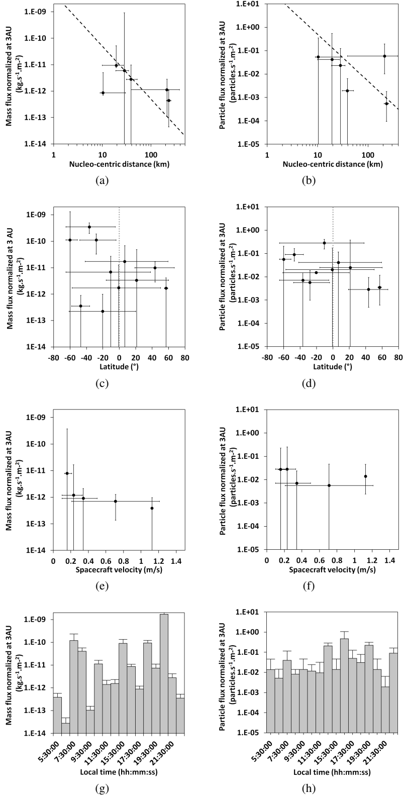
Fig. 6. High phase angle ( 75^{\circ} – 90^{\circ} ) mass fluxes of dust ( left column ) and particle fluxes ( right column ) normalized to the solar distance at 3 AU. a), b) Fluxes plotted versus the distance to the comet center. The data are averaged on nucleocentric distance bins of 10 km. The dashed line represent the 1/d_{\text{comet}}^2 law. c), d) Fluxes plotted versus the latitude. The data are averaged on latitude bins of 10^{\circ} . e), f) Fluxes plotted versus the spacecraft velocity. The data are averaged on velocity bins of 0.1 m/s. g), h) Fluxes plotted versus local time. The error bars represent the standard deviation in each bin.
