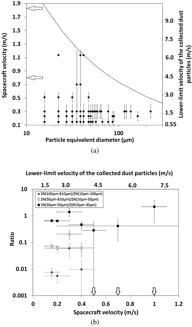
Fig. 11. a) Scatter plot showing the typical size of the collected particles collected at different spacecraft velocities. The arrows represent the collection periods for which no particles have been detected and thus correspond to an upper limit of the size of eventually collected particles (the limit being given by the resolution of the COSISCOPE). In this plot, the particles fragmented on the walls of the funnel are not included. The dashed line represents the v \sim \text{size}^{-0.5} dependence. b) Gray dots: ratio of the number of particles larger than 100 μm/number of particles smaller than 100 μm. White dots: ratio of the number of particles larger than 50 μm/number of particles smaller than 50 μm. The arrows represent null ratios obtained in these two cases for spacecraft velocities larger than 0.5 m/s for which no particles above 50 μm have been collected. Black squares: ratio of the number of particles with sizes comprised between 30 μm and 50 μm/number of particles between 10 μm and 30 μm. In all cases, the error bars represent a 1\sigma error.
