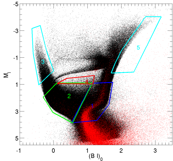
Figure 2. Synthetic CMD with the simulated observational effects (black) with overplotted the observed CMD (red). Bundles are the regions numbered from 1 to 5, see text for details.
