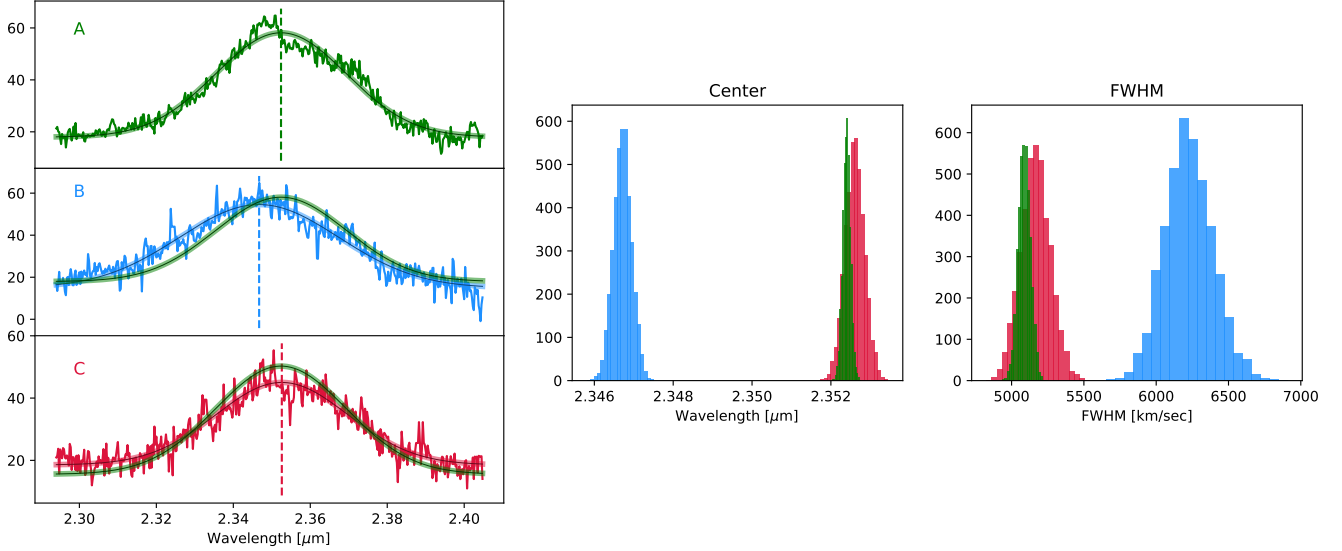
Fig. 2. Comparison of the H\alpha lines of the three components of J1608+2716. Left panels, from top to bottom: A, B, and C components, color-coded as in Fig. 1. Each panel shows the observed emission line scaled to the same flux of component A, and fit with a Gaussian profile plus a constant (shown as a thick solid line with the same color as the corresponding component). The center of the best-fitting Gaussian is reported as a vertical dashed line. For an easy comparison, the fit to component A (the brightest component) is also shown on top of components B and C. Right panels: distributions of the values of centroids and FWHM for the Gaussian fit on 4000 stochastic realizations of the observed spectra, each obtained by injecting noise into the data.
