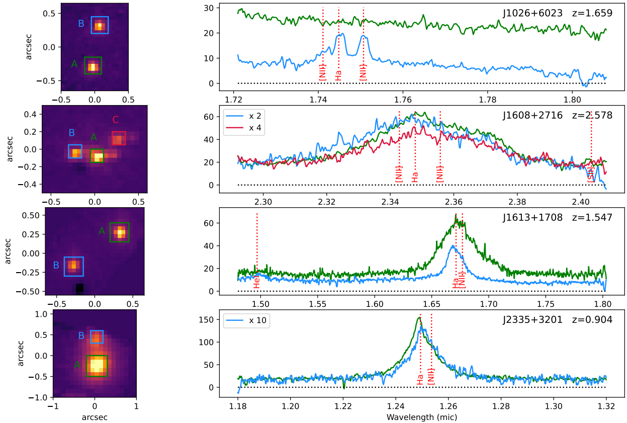
Fig. 1. H\alpha emission line maps (left) and spectra (right) of the systems observed with OSIRIS (the target name and redshift are reported in the right panels). The line maps are oriented with north being up and west to the right. The spectra shown in the right panels have been extracted over the squared apertures marked in the left panels (with the same color-coding). Each component of the systems is labeled as in Table 2. To optimize the visualization, some of the spectra have been multiplied by the factors indicated in the labels. Vertical dotted lines show the position of the main expected emission lines.
