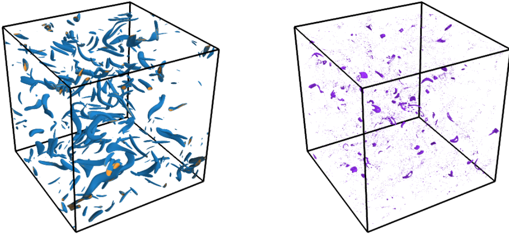
Figure 4. Test particle simulations of the propagation of cosmic rays in a random magnetic field (figures 2 and 8 in [45]); the particles' Larmor radius is 6% of the correlation length of the magnetic field. Left-hand panel: isosurfaces of the strength of a random magnetic field \vec{B} produced by the fluctuation dynamo, B^2/B_0^2 = 12 (blue) and 15 (yellow), with B_0 the root-mean square field strength. The magnetic field is intermittent, its correlation length is about 40 times smaller than the correlation length of the chaotic flow that generates it. Right-hand panel: isosurfaces of the cosmic ray number density in the magnetic field of the left-hand panel at n_{\text{CR}}/n_0 = 3.5 , where n_0 is the mean value of n_{\text{CR}} . The cosmic ray and magnetic field strength distributions are statistically independent. The number density of cosmic ray particles is larger in random magnetic traps between magnetic mirrors. Reproduced from [45]. © 2017 The Authors Published by Oxford University Press on behalf of the Royal Astronomical Society.
