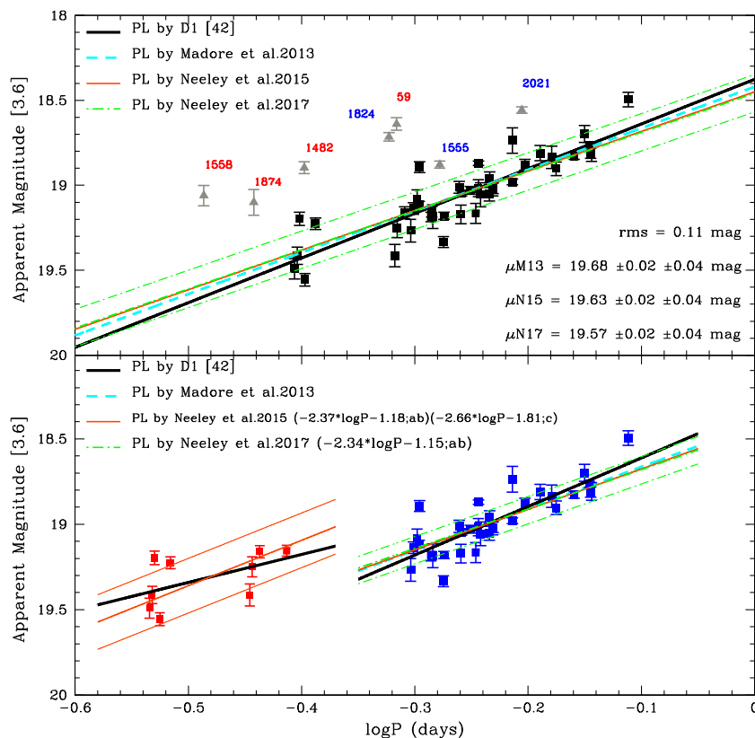
Figure 4. Top: 3.6 \mu\text{m} PL relations defined by the 42 RRLs observed in Sculptor (D1 sample). The periods of the RRC stars have been fundamentalized. The black solid line represents the least-squares fit to the data in Table 1. The triangles are the most problematic stars not used in the least-square fit. Bottom: RRab (blue symbols) and RRC (red symbols) stars are plotted in two PL relations that were computed from the fundamental-mode and the first-overtone pulsators separately. In both panels, the cyan (dashed), orange (thin solid), and green (dash-dot) lines mark Madore et al. (2013), Neeley et al. (2015), and Neeley et al. (2017) PL relations, respectively. We show only \pm 2\sigma the deviation lines of the Neeley et al. (2017)’s PL; the dispersions of the other PL relations are similar or slightly broader.
