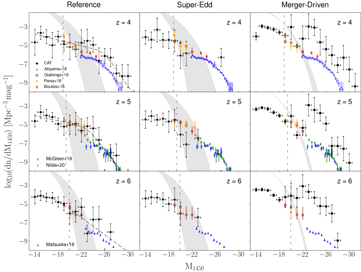
Figure 9. The AGN UV LFs at z = 4, 5 , and 6 (from top to bottom). Each column shows the results obtained in one of the three CAT models: the reference model (left panels), the super-Edd model (central panels) and the merger-driven model (right panels). Black data points represent the predicted AGN LFs, properly corrected for obscuration as described in the text. The black dashed line shows the best fit for the Reference model. The grey shaded area encloses the region between the intrinsic and the dust corrected galaxy UV luminosity function predicted by each model at the corresponding redshift. Coloured data represent the observational constraints on the AGN LF obtained by Parsa et al. (2018, orange circles), Boutsia et al. (2018, red diamonds), Giallongo et al. (2019, brown squares), by the SHELLQs survey (Matsuoka et al. 2018), the CFHT Legacy Survey (McGreer et al. 2018), and the Hyper Suprime-Cam Wide Survey (Akiyama et al. 2018; Niida et al. 2020) (blue triangles and green diamonds). The vertical black dashed lines show the JWST luminosity limit at each redshift predicted by Griffin et al. (2020).
