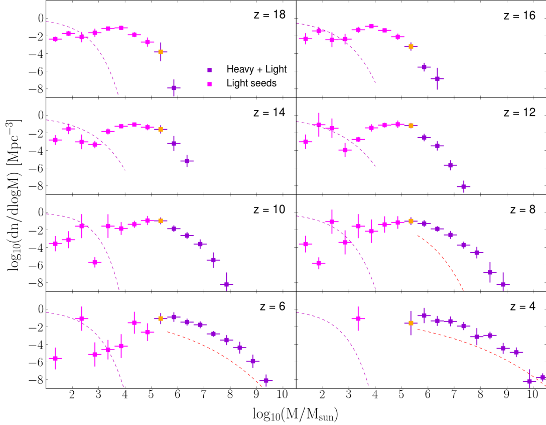
Figure 6. Same as Fig. 5 but for the merger-driven accretion model (see Section 2.4.2). Here we show with violet data points the mass bins above 10^5 M_\odot since, unlike the previous models, they are now populated by both light and heavy BH seed descendants. Distributions (data points with error bars) are compared with best fits obtained for the reference model (dashed lines).
