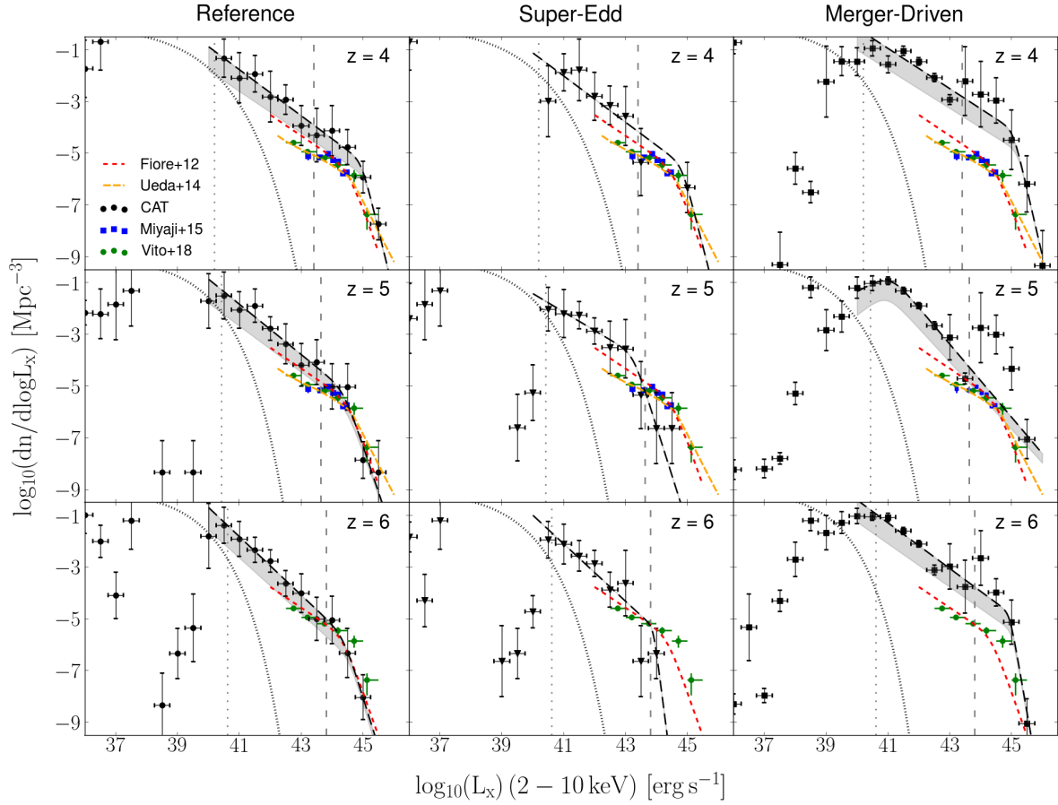
Figure 10. The AGN LFs in the [2 - 10] keV X-ray energy band at z = 4, 5 , and 6 (from top to bottom). Each column shows the results obtained in one of the three models examined: the reference model (left panels), the super-Edd model (central panels) and the merger-driven model (right panels). In the left and right panels, the grey shaded regions show how the best-fit distributions change assuming the fraction of absorbed AGNs proposed by Ueda et al. (2014). In each panel, the black dotted line represents the X-ray LF associated with star formation in the host galaxies at the same redshift, that we have estimated using the relation proposed by Fornasini et al. (2018, see text). Coloured data represent the observational results by Fiore et al. (2012, red dashed line, z = 4.5, 6 ), Ueda et al. (2014, orange dashed line, 4 < z < 5 ), Miyaji et al. (2015, blue squares, 3 < z < 5.8 ) and Vito et al. (2018, green circles, 3.6 < z < 6 ). The dashed and dotted grey vertical lines represent the luminosity limits estimated by Griffin et al. (2020) for, respectively, Athena and Lynx.
