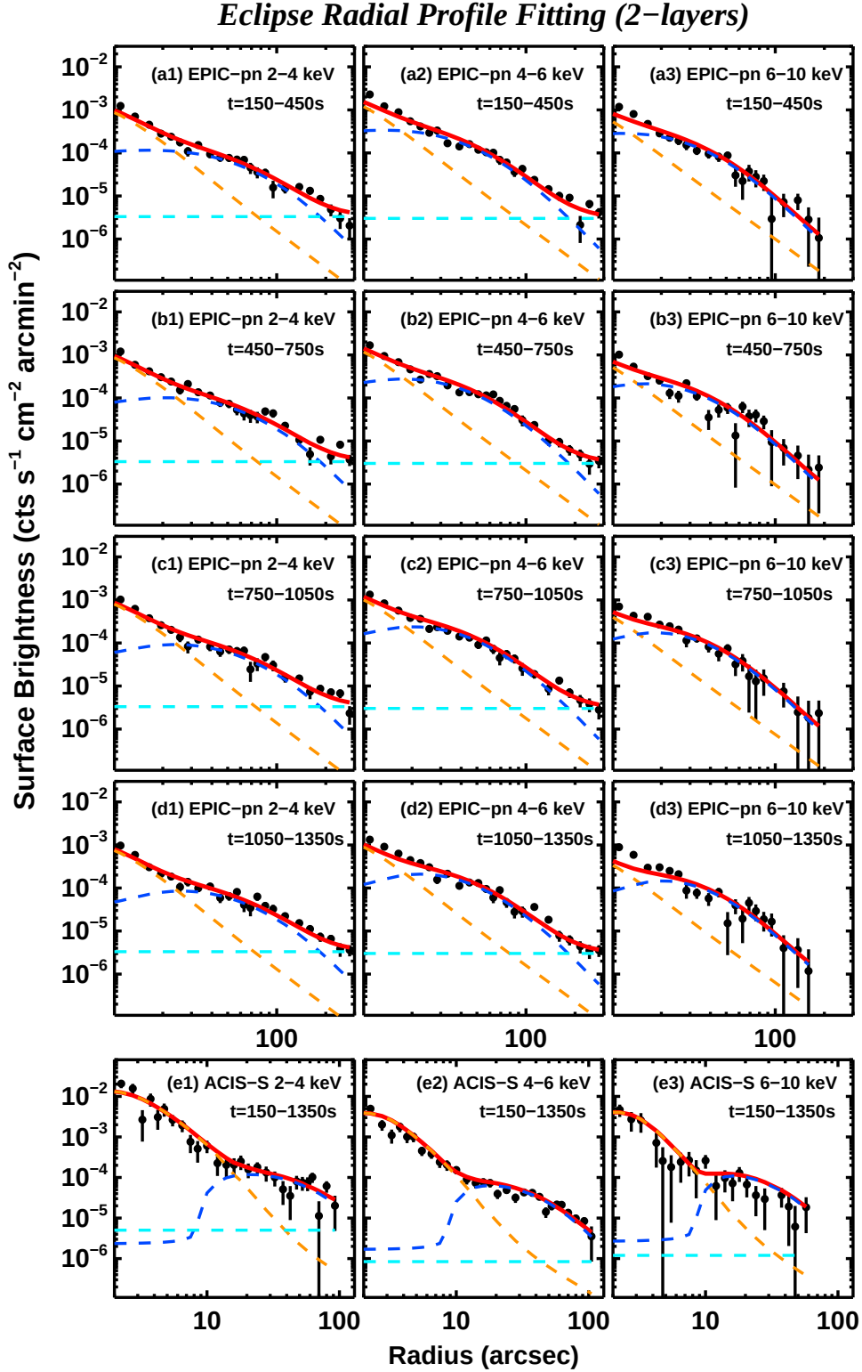
Figure A1. A simultaneous fit to the non-eclipse radial profiles in Fig.6 and eclipse radial profiles in this figure, using the 2-layer scenario with the COMP-AC-S grain population in every layer. The type of instrument, energy band and time interval (relative to the eclipse ingress time) have all been labeled in every panel. The orange dash line is for Layer-1, blue is for Layer-2, and cyan is for the halo wing component. The red solid line is for the total halo model. There is no PSF component in the radial profile as the primary source is eclipsed. The best-fit parameters can be found in Tables 2 and 4.
