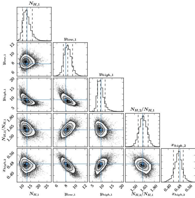
Figure 8. The bayesian parameter estimation using MCMC sampling for the 2-layer scenario (Fig.6 1st row) with the COMP-AC-S dust grain model. Each histogram shows the marginalized distribution, the three dash lines from left to right indicate the 10th, 50th and 90th percentiles of the samples, respectively. For clarity, we performed the linear conversion: y_{low,1} = (1 - x_{low,1}) \times 10^2 , y_{high,1} = (1 - x_{high,1}) \times 10^4 . The blue solid lines indicate the best-fit values for the minimum \chi^2 method (see Table 2). The results for 3 and 4 dust layers are shown in Fig.B1-B2.
