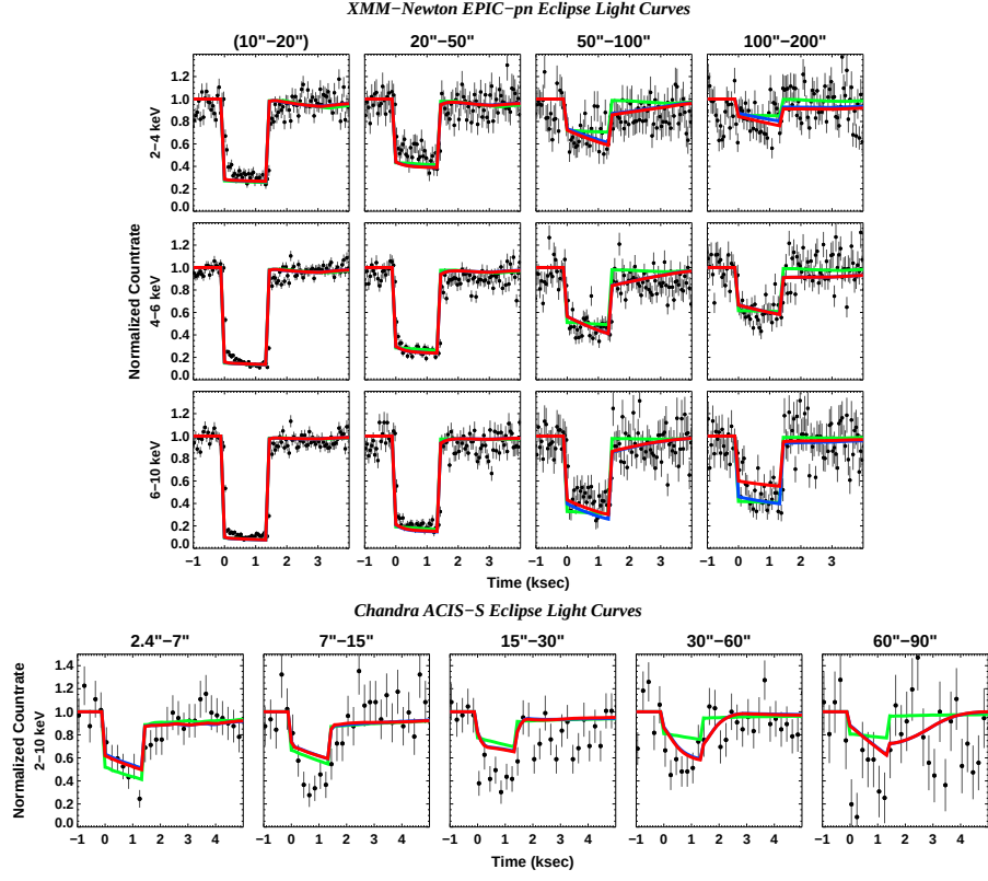
Figure C1. Similar to Fig. 7, but using the GM2 dust grain configuration, i.e. replacing the dust grain model with the MRN grain population for all dust layers.
