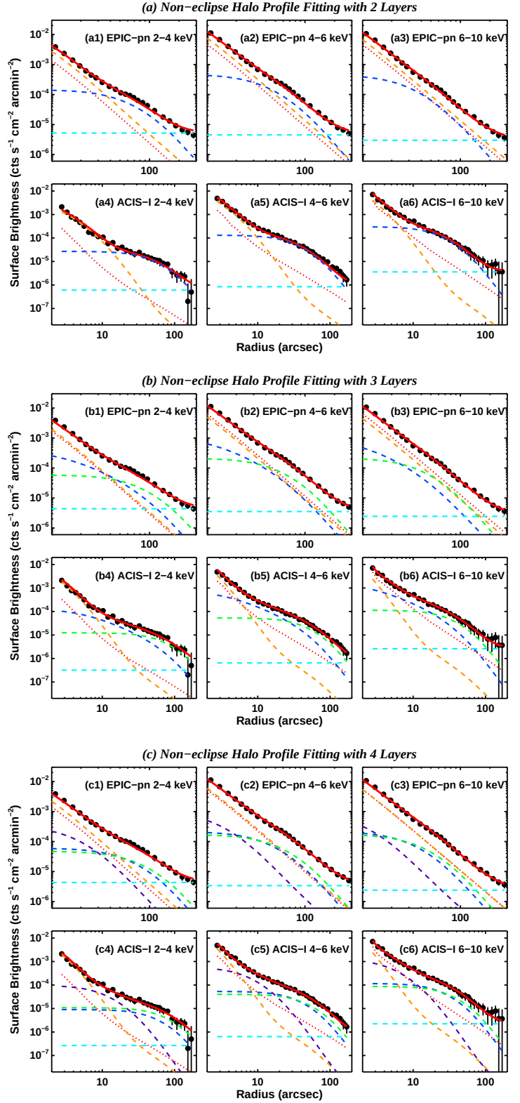
Figure 6. Dust models with 2, 3 and 4 distinct layers along the LOS. In each row, the left-side cartoon shows each layer's position and parameters. The best-fit results using the COMP-AC-S dust grain model (see Section 5.2.1) are shown on the right side, with dash lines indicating the contribution from every dust scattering component (cyan dash line is the wing component), and the dotted line indicating the instrumental PSF. The results of simultaneous fitting to the eclipse halo profiles using the same model can be found in Fig. A1-A3.
