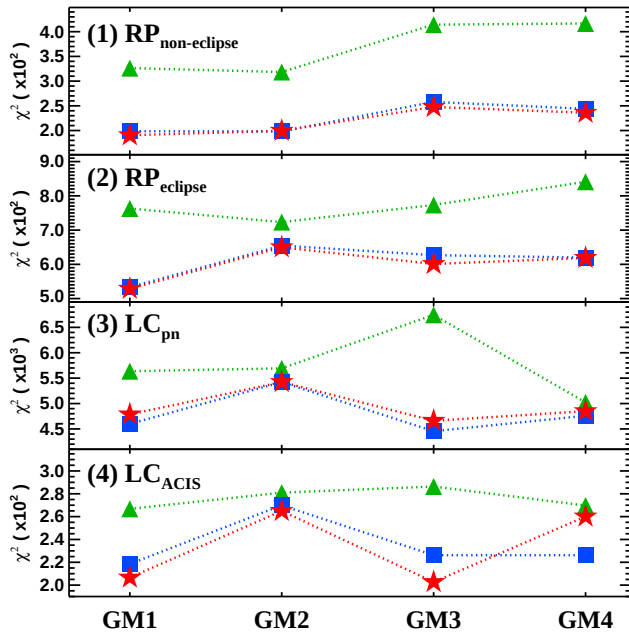
Figure 9. Comparison of different \chi^2 values in Table 4. The green triangle, blue square and red star symbols indicate the results for the 2, 3 and 4 dust-layer scenarios, respectively.
