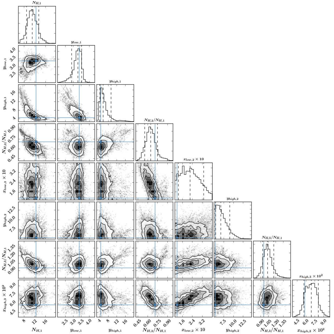
Figure B1. Similar to Fig. 8, but for the MCMC sampling under the 3-layer scenario with the COMP-AC-S dust grain model. The meaning of each parameter can be found in Fig. 6. For clarity, we performed the linear conversion: y_{low,1} = (1 - x_{low,1}) \times 10^2 , y_{high,1} = (1 - x_{high,1}) \times 10^3 , y_{high,2} = (1 - x_{high,2}) \times 10^2 . The blue solid lines indicate the best-fit values using the minimum \chi^2 method.
