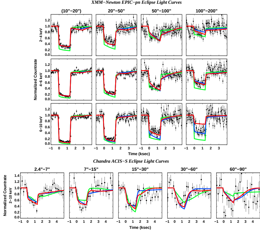
Figure C2. Similar to Fig. 7, but using the GM3 dust grain configuration, i.e. using the replacing the dust grain model with the ZDA04 COMP-NC-B grain population for all the dust layers except the one local to the source.
