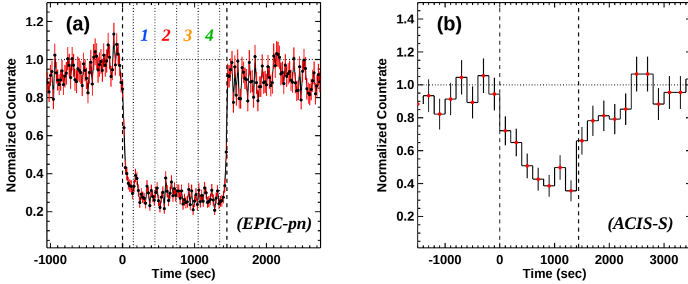
Figure 2. The combined 2-10 keV eclipse light curves of AX J1745.6-2901 based on the observations listed in Table 1. Panel-a shows the results for XMM-Newton EPIC-pn, where the source extraction region is 20-100 arcsec and the light curve binning time is 20 s. The eclipse phase is divided into 4 time intervals, where the corresponding radial profiles can be found in Fig.3. Panel-b shows the results for Chandra ACIS-S, where the source extraction region is 2.4-20 arcsec and the binning time is 100 s. Background count rates have been subtracted, which were determined from observations during which AX J1745.6-2901 was in quiescence (see Table B1, B2 in J17). t = 0 s is the eclipse ingress time.
