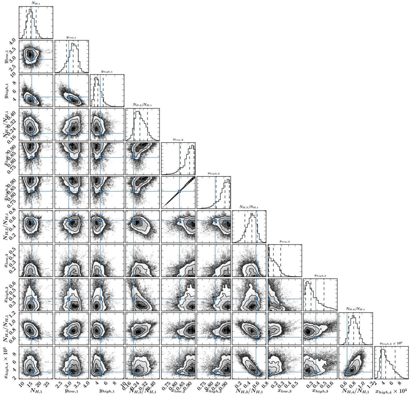
Figure B2. Similar to Fig. 8, but for the MCMC sampling under the 4-layer scenario with the COMP-AC-S dust grain model. The meaning of each parameter can be found in Fig. 6. For clarity, we performed the linear conversion: y_{low,1} = (1 - x_{low,1}) \times 10^2 , y_{high,1} = (1 - x_{high,1}) \times 10^3 . The blue solid lines indicate the best-fit values using the minimum \chi^2 method.
