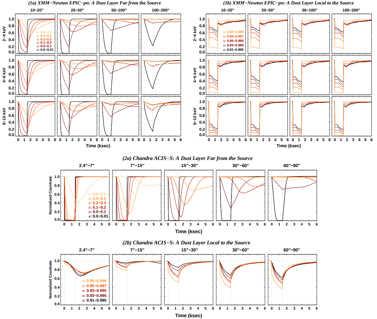
Figure 5. The simulated eclipse light curves of the dust scattering halo. Panel-1a shows the results for XMM-Newton EPIC-pn for a dust layer far from the source. In each sub-panel there are 6 lines showing the results for a dust layer located within a fractional distance of 0.0-0.01, 0.0-0.1, 0.1-0.2, 0.2-0.3, 0.4-0.5, 0.8-0.9, respectively. These sub-panels clearly reveal the dependence of the eclipse light curves on the energy band and source extraction region (i.e. radial range). Panel-1b is similar but for a dust layer local to the source, within a fractional distance of 0.91-0.995, 0.93-0.995, 0.95-0.995, 0.95-0.997, 0.95-0.999, respectively. Panel-2a,2b show the results of simulation for Chandra ACIS-S.
