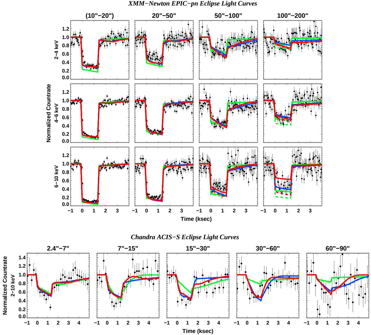
Figure 7. Posterior comparison between the real eclipse light curves observed by XMM-Newton EPIC-pn and Chandra ACIS-S, and the simulated eclipse light curves from the best-fit models with the COMP-AC-S dust grain model for different dust-layer scenarios (Fig. 6, Table 2). Green, blue and red lines indicate the results for the 2, 3 and 4 dust-layer scenarios, respectively. The solid line assumes that the halo wing does not respond to the eclipse signal, while the dash line assumes that the halo wing responds instantaneously to the eclipse signal. In EPIC-pn the 10-20 arcsec region was slightly contaminated by the photon pile-up effect, so we only plot them for the purpose of comparison. The results for the other dust grain models tried in this paper can be found in Fig. C1-C3.
