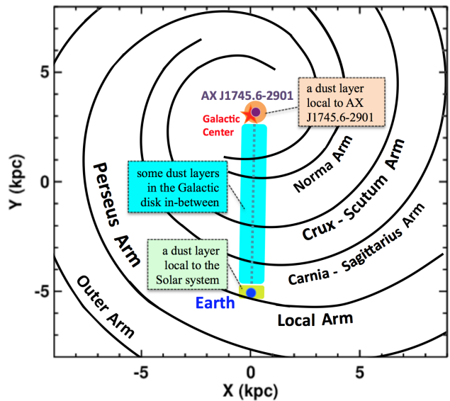
Figure 10. Dust distribution along the LOS of AX J1745.6-2901, as suggested by the best-fit 3-layer and 4-layer models in Table 2, assuming it is in the GC. The schematic of Milky Way’s spiral arms, as shown in Nakanishi & Sofue (2016), Reid et al. (2009), Caswell & Haynes (1987) (also see the review by Bland-Hawthorn & Gerhard (2016)), are also plotted for comparison. Compared to the 2-layer model in Figure 15 of J17, now we identified a third dust layer in the Solar neighbourhood (see Section 6.3), although the second dust layer (cyan region) in the Galactic disk is still poorly resolved.
