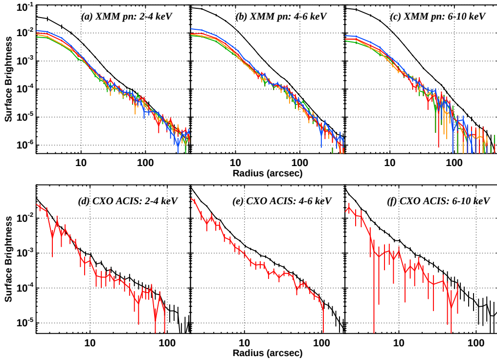
Figure 3. Comparison of the radial profiles of AX J1745.6-2901 during the non-eclipse and eclipse phases for the energy bands of 2-4, 4-6 and 6-10 keV. In Panel-a,b,c the black line is the radial profile during the non-eclipse phase as being observed by XMM-Newton EPIC-pn. The blue, red, orange and green profiles are the radial profiles observed during the four time intervals within the eclipse phase in Fig.2a. The central 20 arcsec was contaminated by photon pile-up; we only plot them for the purpose of comparison. In Panel-d,e,f the black line is the radial profile observed during the non-eclipse phase by Chandra ACIS-I, and renormalized to the brightness of those observed during the ACIS-S observation. We did not directly use the non-eclipse radial profiles from ACIS-S because of the smaller radial coverage in the sub-array mode, and they are consistent with these ACIS-I radial profiles (see J17). The red line is the eclipse radial profiles observed by Chandra ACIS-S. Background radial profiles were determined from observations during which AX J1745.6-2901 was in quiescence (see Table B1, B2 in J17), and were subtracted from these radial profiles.
