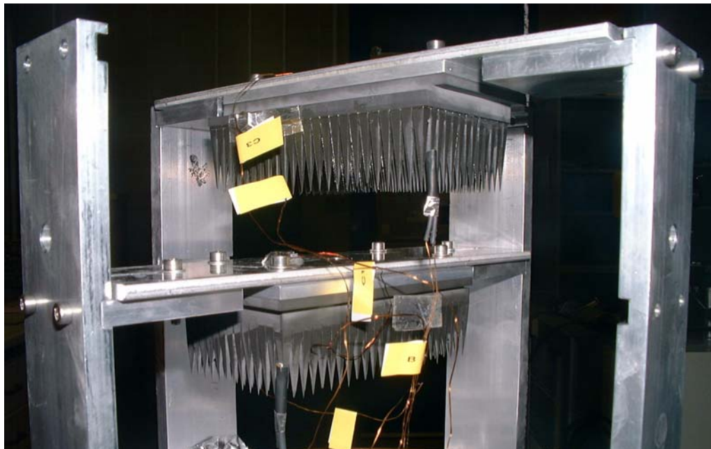
Figure 27 panels mounted on supports before dismounting
