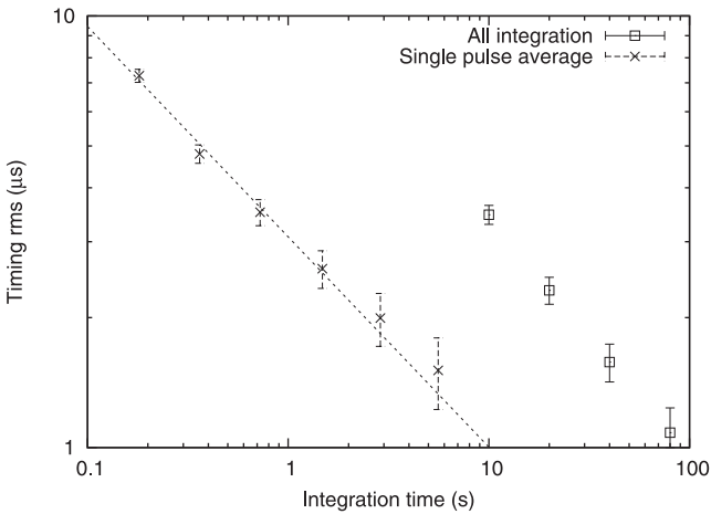
Figure 17. Timing rms of averages based on different numbers of bright subpulses, compared with the rms from integrations of all periods. The dashed line shows a power-law modelling with a fitted index of -0.49 \pm 0.02 . Note that an integration of 10 s corresponds to roughly 600 pulses.
