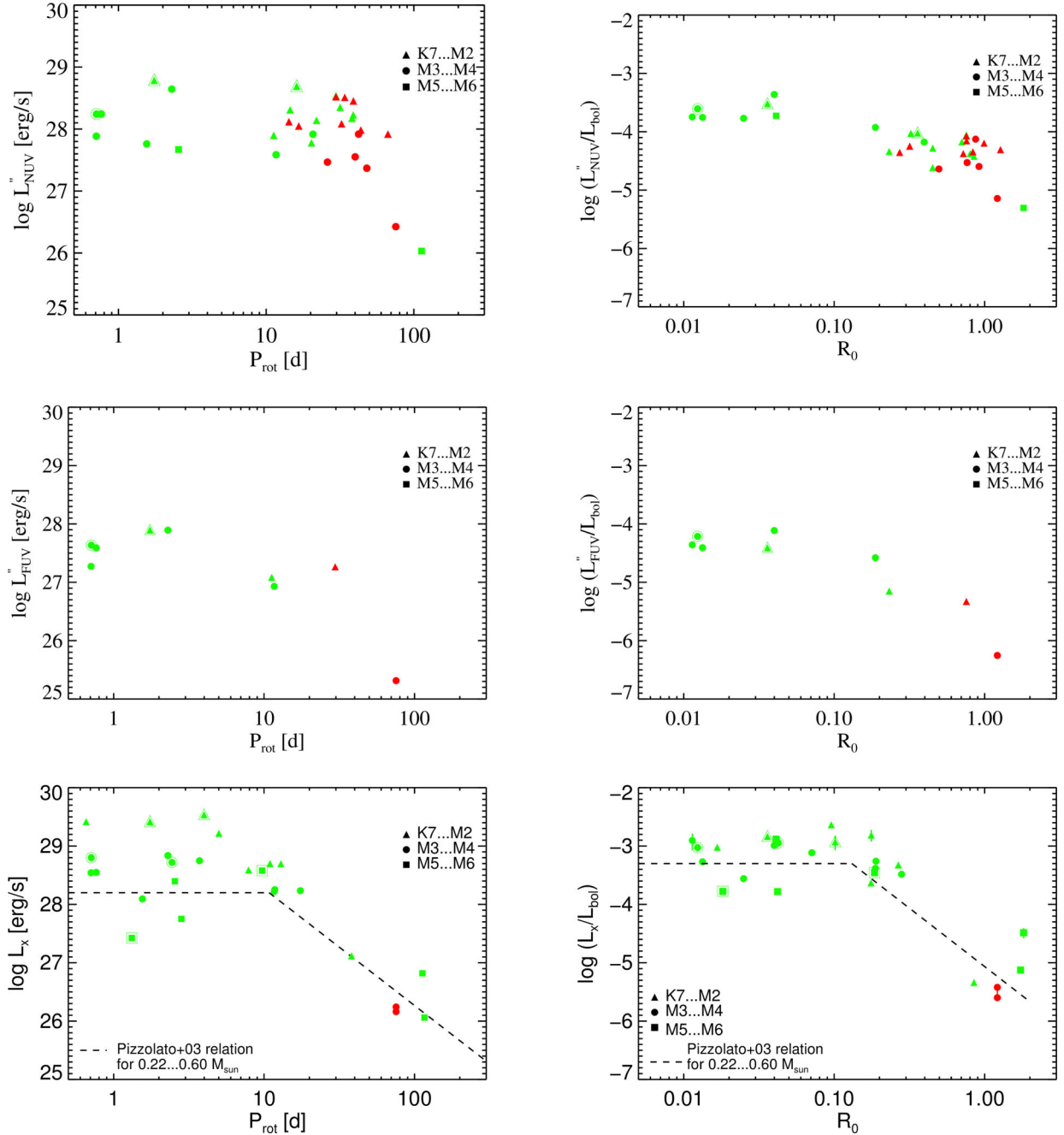
Figure 15. K2 rotation periods combined with archival NUV (top), FUV (middle) and X-ray (bottom) data for the campaign C0–C4 Superblink M stars. In the left-hand panels, luminosities versus rotation period, in the right-hand panels activity indices versus Rossby number. Periods flagged ‘?’ are shown in red, unresolved binaries are represented with large annuli.
