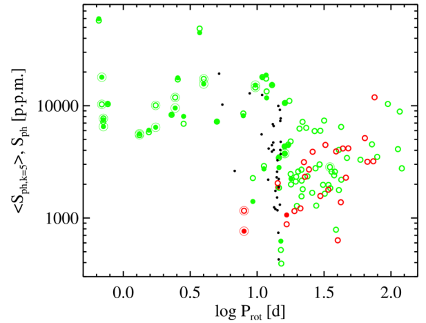
Figure 12. Magnetic activity indices defined by Mathur et al. (2014) versus period for the K2 Superblink star sample, compared to the subsample of 34 Kepler field M dwarfs studied by (Mathur et al. 2014, black dots). Green and red symbols represent periods flagged ‘Y’ and ‘?’, respectively. Filled circles denote \langle S_{\text{ph},k=5} \rangle values and open circles the S_{\text{ph}} values. See the text in Section 7.3 for details on the definition of these indices. Large annuli mark binaries.
