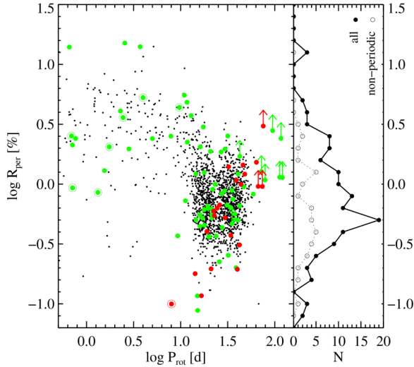
Figure 11. Period versus amplitude for the K2 Superblink M dwarf sample (large, coloured circles) compared to the Kepler field M dwarfs from (McQuillan et al. 2013, small, black dots). For our K2 sample, we distinguish reliable periods (green) and questionable periods (red). Banner on the right: histogram of R_{\text{per}} for the full K2 Superblink star sample (solid line) and for the subsample classified as non-periodic (flag ‘N’). As in the other figures, binaries in our K2 Superblink sample are marked with large annuli.
