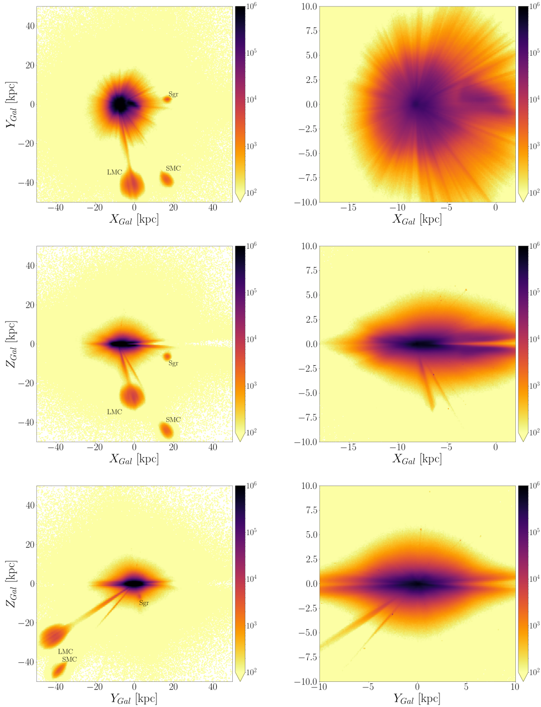
Fig. 7. StarHorse density maps (from top to bottom: XY , XZ , and YZ ) in galactocentric coordinates. Left column : 100 kpc wide cube centred on the Galactic centre, while right column : zooms into a 20 kpc wide cube centred on the Sun.
