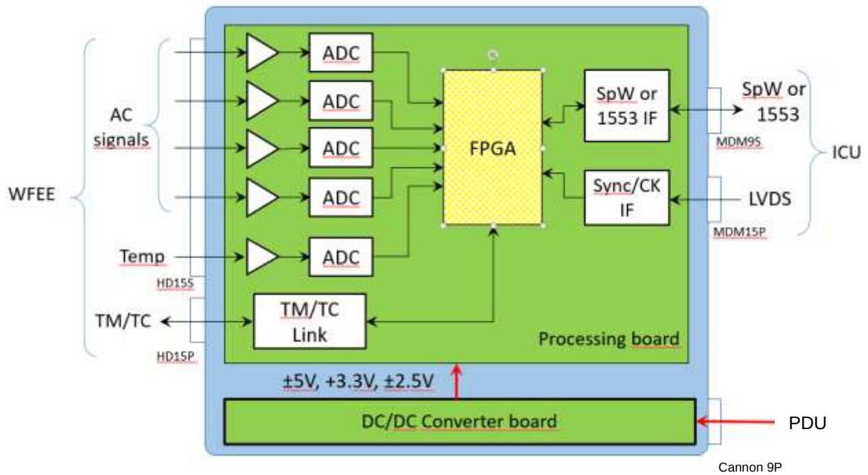
Fig. 9. Block diagram of the WBEE.
