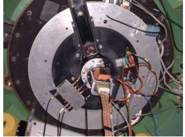
Fig. 5. The PC-ICCD mounted at the 182 cm cima Ekar telescope. Below: observation of the Crab nebula and fourier analysis of the photons from the Crab pulsar.
