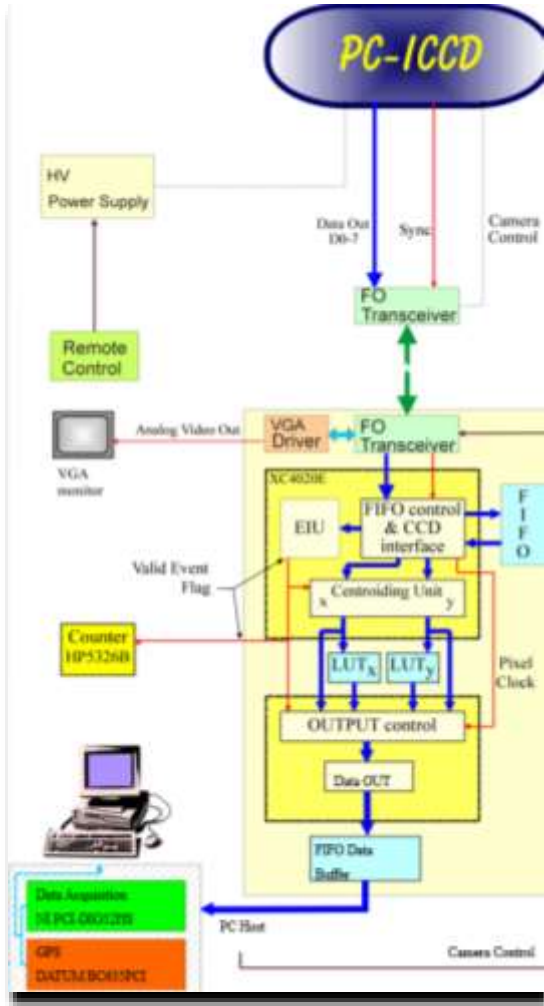
Fig. 4. Block diagram of the ICCD optimized for the optical range
