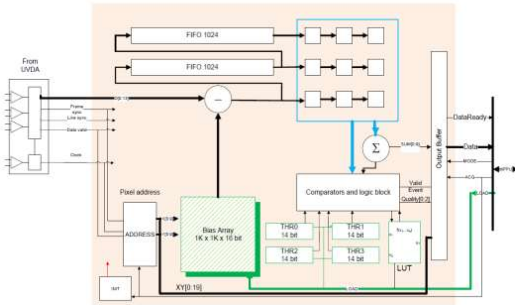
Fig. 7. Block diagram of the PCU IP core.
