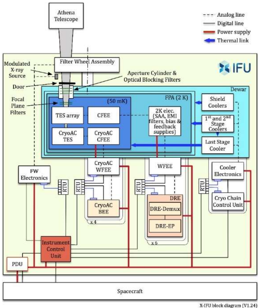
Fig. 8 . Block diagram of the ATHENA XIFU.
