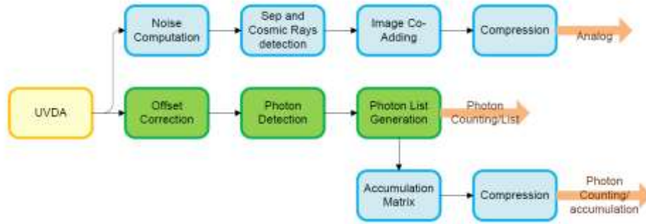
Fig. 6. Block diagram of the UVDA on-board processing. The green box have been implemented in the IP core PCU, along with the UV flux monitoring flags.
