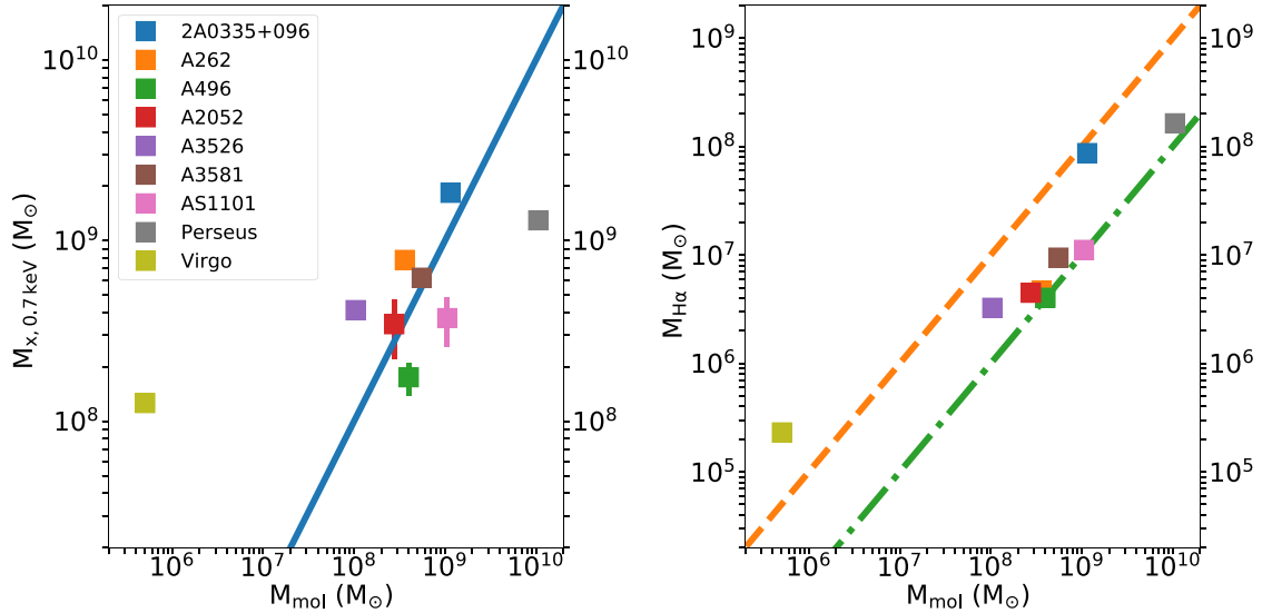
Figure 2. Left-hand panel: The X-ray emitting gas against molecular mass. The blue line indicates where the molecular mass would match the soft X-ray mass. Right-hand panel: The mass of H \alpha component against molecular mass. The orange dash line has a constant M_{\text{H}\alpha}/M_{\text{mol}} ratio of 0.1 and the green dash-dot line has a ratio of 0.01. The uncertainties in the mass of molecular and H \alpha emitting gas is smaller than the marker size.
