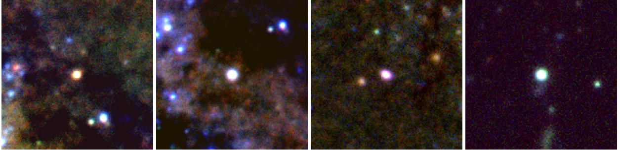
Fig. 9. RGB thumbnails from VST data of star cluster candidates from Beasley & Sharples (2000) that did not pass our selection criteria for GC candidates. Starting from left: B13 and B14 (close to galaxy dusty regions), and B29 and LA11 (likely background galaxies). Thumbnails are 15'' on each side.
