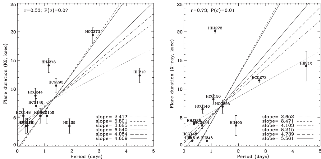
FIGURE 4 Flare duration in optical (left panel) and X-rays (right panel) vs. stellar rotation period. For each data point, we show the name of the star. The lines mark six linear fits performed with the IDL routine SIXLIN . The resulting slopes are indicated in the bottom right corner. In the top left corner we also show the Spearman's rank correlation coefficient and the significance of its deviation from zero. In both cases the most rapidly rotating stars in our sample host short flares
