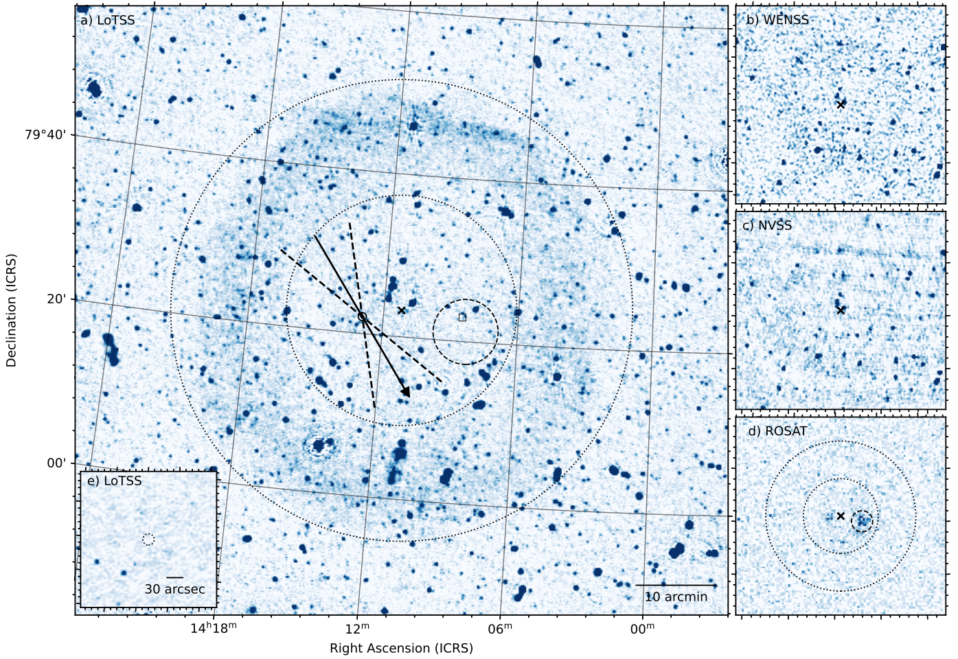
Fig. 1. Possible Calvera supernova remnant. (a) Radio emission from the diffuse ring at 144 MHz in the LOFAR HBA LoTSS imaging mosaic ( 1^{\circ}25' \times 1^{\circ}25' field of view, 20'' resolution). The location of Calvera is indicated with a circle, with the arrow representing the Halpern & Gotthelf (2015) proper motion from 10 kyr in the past to 10 kyr into the future. The dashed lines indicate the propagated 1\sigma positional uncertainty due to proper motion. The cross sign indicates the estimated center of the diffuse ring, with the dotted circles representing the inner and outer radii. The dashed circle ( 4' radius) denotes the location of the diffuse X-ray emission seen by Zane et al. (2011) from 1RXS J140818.1+792113, with the square indicating the location of H\alpha emission. (b) The diffuse ring in the Westerbork Synthesis Radio Telescope WENSS survey imaging at 325 MHz and (c) the Very Large Array NVSS survey at 1.4 GHz. Both panels have a 1^{\circ}25' \times 1^{\circ}25' field of view and an identical pointing and orientation to panel a. (d) The 0.1–2.4 keV X-ray image from RASS (Voges et al. 1999), with the ring center and inner outer radii of the radio ring denoted by the cross and dotted circles. The dashed circle encircles the emission from 1RXS J140818.1+792113. (e) A 2' \times 2' section of the 6'' resolution LoTSS imaging mosaic at the location of Calvera, indicated with the dotted circle ( 10'' radius).
