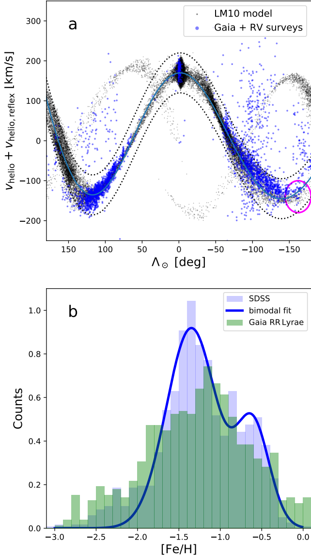
Figure 3. a: Radial velocities of the cleaned STREAMFINDER sample, as measured in public spectroscopic surveys. The behavior of the younger tidal arms in the ( < 3 \text{ Gyr} ) LM10 model are also shown, along with a sinusoidal fit to these particles (solid line). The magenta circle highlights the nearby leading arm. b: The metallicity distribution of the SDSS-Segue stars (blue) in the sample (and that also lie between the dotted lines in panel a) is compared to the Gaia RR Lyrae sample (green). The blue line shows a bimodal Gaussian fit to the Segue sample.
