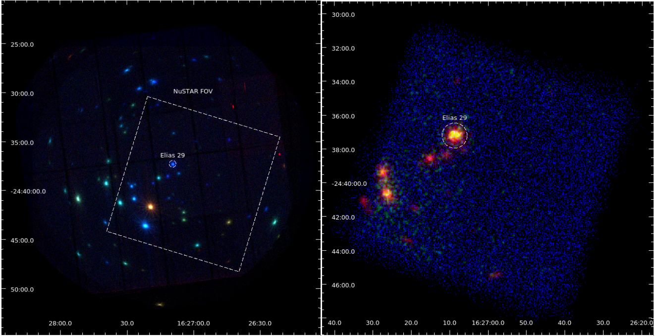
Fig. 1. Left panel: color-coded image of the EPIC data integrated over the entire observation (red: 0.3–1.0 keV; green: 1.0–3.0 keV; blue: 3.0–8.0 keV). The square indicates the FOV of the NuSTAR observation. Right panel: color-coded image of the NuSTAR data integrated over the entire observation (red: 3–10 keV; green 10–40 keV; blue 40–60 keV). In both images a circle indicates the position of Elias 29.
