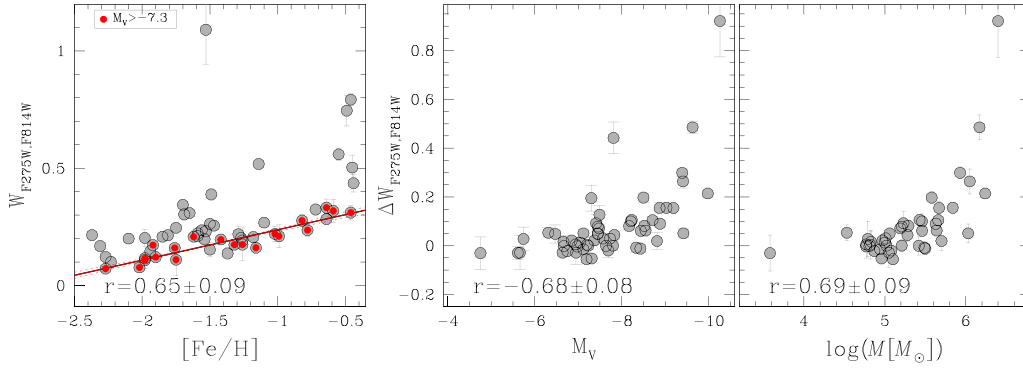
Figure 21. The left-hand panel shows the intrinsic RGB width, W_{F275W, F814W} , as a function of metallicity of the host GC. The red line is the best-fitting straight line for clusters with M_V > -7.3 that we have represented with red dots. The residuals of the RGB width with respect to the best-fitting line, \Delta W_{F275W, F814W} , are plotted against the absolute visual magnitude and the cluster mass in the middle and the right-hand panels, respectively. The Spearman's rank correlation coefficient and the corresponding uncertainty are reported in each panel. The outlier point refers to \omega Centauri.
