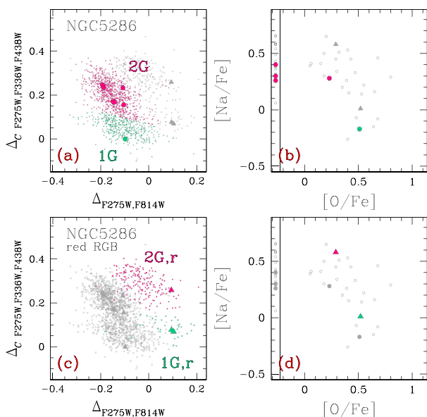
Figure 19. In the chromosome map of NGC 5286, shown in panel (a) only stars from the blue-RGB are used, i.e. those coloured black in Fig. 12. Aqua and magenta colours highlight 1G and 2G stars, respectively, with stars also studied spectroscopically are represented by large filled symbols and whose [Na/Fe] versus [O/Fe] plot from Marino et al. (2015) is shown in panel (b). Finally, in panel (c) the red-RGB stars are coloured either aqua or red for being considered the first or the second generation (1G,r and 2G,r) of the iron-rich population, while panel (d) shows the corresponding [Na/Fe] versus [O/Fe] from Marino et al. (2015).
