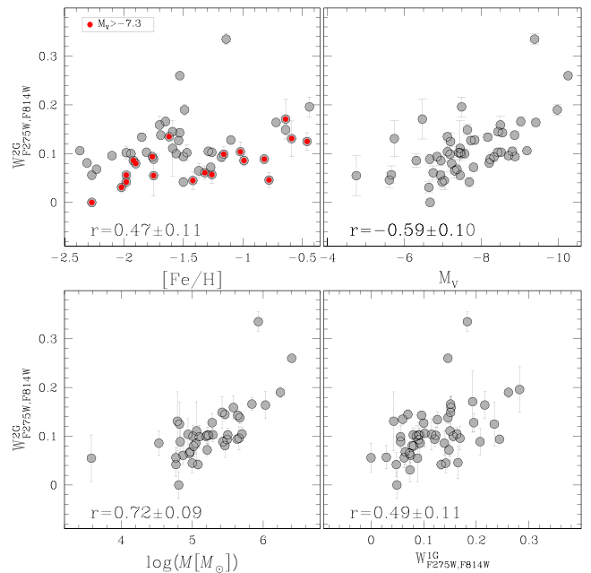
Figure 23. The intrinsic width W_{F275W, F814W}^{2G} of the 2G stars as a function of cluster metallicity and absolute magnitude (upper-left and -right panels, respectively), and as a function of the cluster mass and of the intrinsic width of 1G stars (lower-left and -right panels, respectively). Symbols are like in Fig. 20. The Spearman's rank correlation coefficient and the corresponding uncertainty are indicated in each panel.
