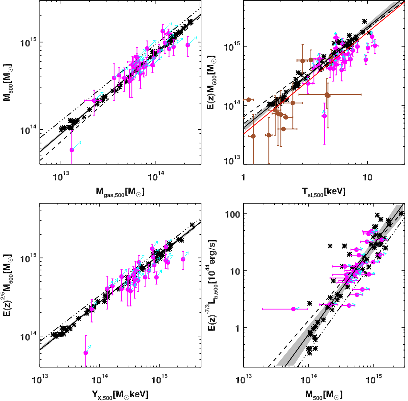
Figure 2. Comparison between scaling relations at z = 0 and those derived from local observations ( z < 0.25 ). In clock-wise order, we plot the M - M_g , M - T_{sl} , L - M , and M - Y_X relations. The observational data are taken from Mahdavi et al. (2013) and Mahdavi et al. (2014) (magenta), and Lieu et al. (2016) (brown). They are shown with 1\sigma error bar. The cyan arrows associated with the Mahdavi et al. points represent the change of the quantities after correcting (i) the total mass by 25 per cent as suggested by Hoekstra et al. (2015) and (ii) the other quantities by the amount estimated within our AGN sample (see the text for details). In each panel, the solid black line represents the best-fitting relation of the AGN sample shown with black asterisks; the grey shaded area is the associated 1\sigma scatter around the best fit; the dashed and dashed-dotted lines represent the best-fitting relations of the NR and CSF runs, respectively. The luminosities are bolometric, none of the simulated and observed quantities is core-excised, and the observed data are rescaled to the cosmology adopted in the simulation.
