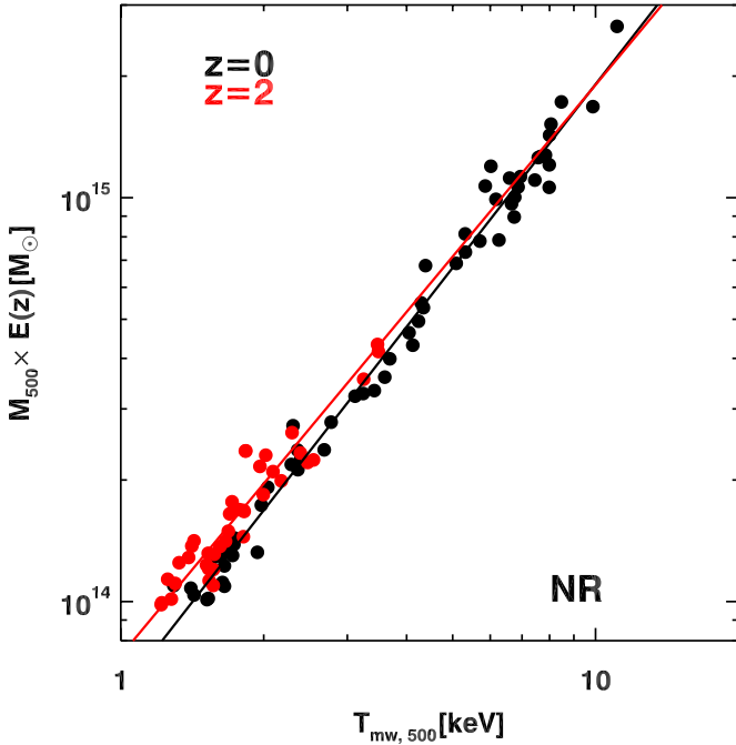
Figure 8. Redshift evolution of the M_{500} - T_{\text{mw}} scaling relation. The result is shown for the NR simulation at redshifts z = 0 (black) and z = 2 (red). The solid lines are the best-fitting relations corresponding to each redshift.
