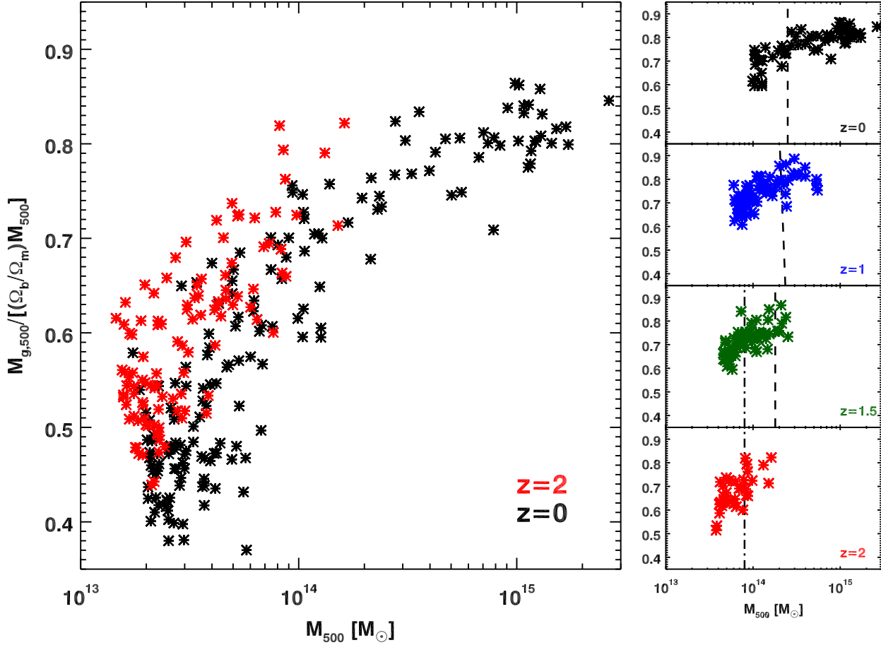
Figure 7. In the large panel we show the baryon fraction of the AGN runs at z = 0 (black) and z = 2 (red) normalized for its cosmic value. All clusters identified in the 29 Lagrangian regions with mass M_{500} above 2 \times 10^{13} M_{\odot} are presented to display the rapid decrease in gas fraction in low mass systems. In the smallest panels at the right, we separately show the objects at z = 0, 1, 1.5 and z = 2 , but only those above the mass limit chosen as threshold ( M_{500} = 10^{14} E(z)^{-1} M_{\odot} ). We indicate the mass limits of the current SPT selection with the dashed-line and that of the future SPT-3G with the dotted-dashed line.
