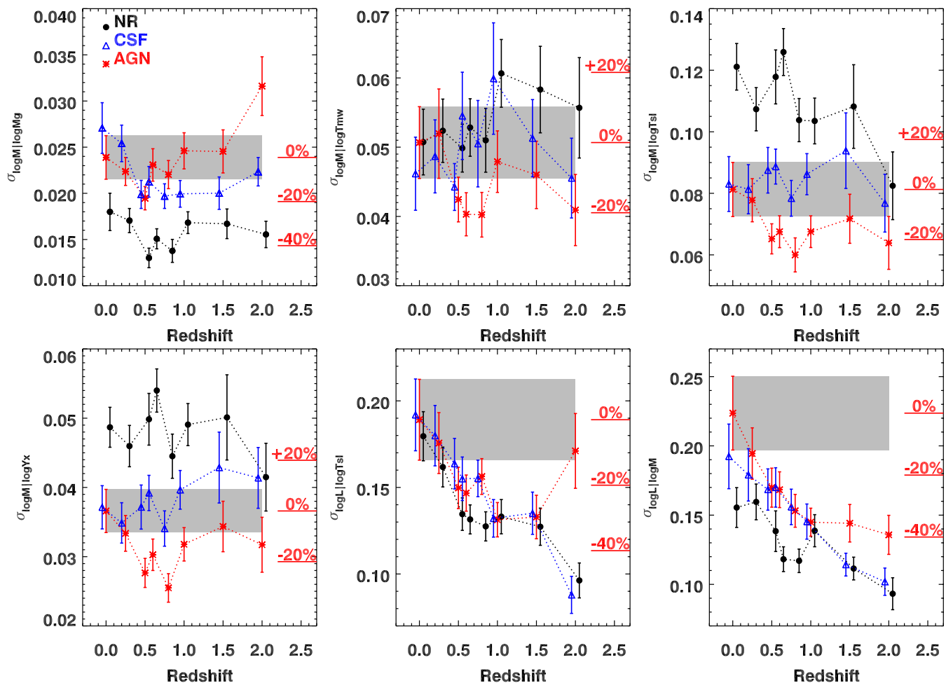
Figure 9. The evolution of intrinsic scatter for M - M_g , M - T_{mw} , M - T_{sl} , M - Y_x , L - T_{sl} , and L - M is shown (from left to right, from top to bottom) as function of redshift and for the three simulated runs. The error bars represent the 1\sigma error, and the grey shaded area stands for the 68% uncertainty of the AGN intrinsic scatter at z = 0 .
