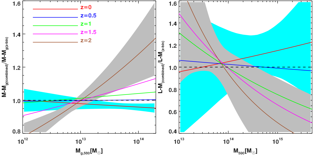
Figure 11. We report, for the AGN sample, the ratio for the M - M_g (left) and L - M (right) between the scaling relations of the combined sample derived via Eq. 11 (best-fitting parameters in Table 5) and the scaling relations previously found in single redshift bins (best-fitting parameters in Tables 2 and 3). The shaded area shows the 68.3% uncertainties for two cases: z = 0 (cyan) and z = 2 (grey). The red, blue, green, magenta, and brown lines refer to the specific comparison at the z bins equal to z = 0, 0.5, 1, 1.5 , and z = 2 , respectively.
