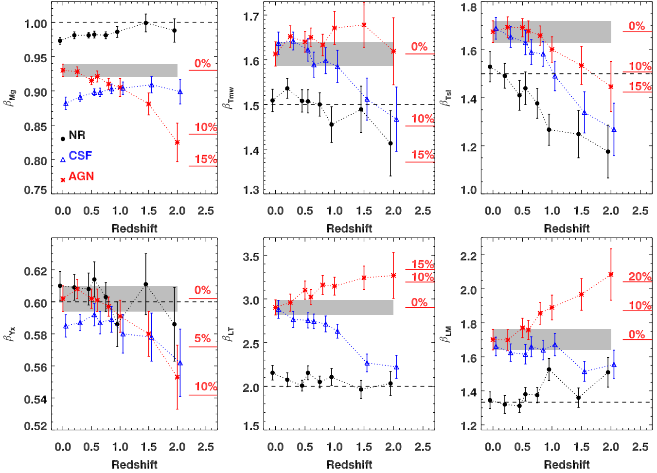
Figure 5. We show the slope value for M - M_g , M - T_{mw} , M - T_{sl} , M - Y_X , L - T_{sl} , and L - M shown from left to right, top to bottom, respectively, as a function of redshift. In each panel, the NR, CSF, and AGN runs are represented by the black circles, open blue triangles, and red asterisks. The dashed black lines represent the self-similar evolution of the slopes. The error bars represent 1\sigma of the \beta parameter. The grey shaded area shows its value at z = 0 for the AGN sample. In this run, we notice that the slopes at redshifts z < 1 agree within 1\sigma with the z = 0 value, while at higher redshifts they can significantly deviate. Some variations from the z = 0 value of the AGN sample are reported with red horizontal lines on the right part of the plots.
