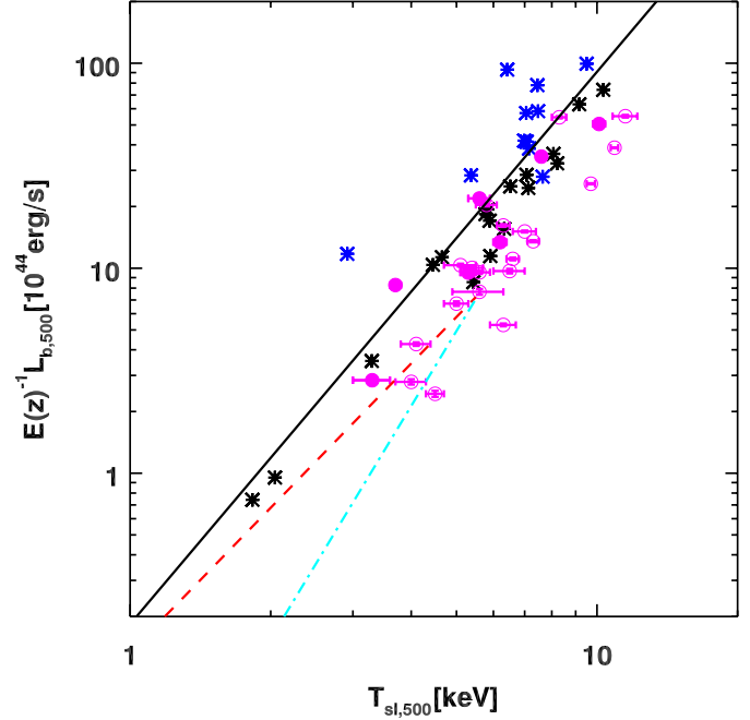
Figure 4. The z = 0 AGN simulated luminosity-temperature relation is shown in blue and black asterisks, respectively, for cool-core and non-cool-core systems (Rasia et al. 2015). For comparison, the cool-core and non-cool-core clusters observed by Mahdavi et al. (2013) are reported with filled and open magenta circles, respectively. The solid line is the best-fitting simulated L - T relation, and the two dashed lines represent the results taken from Gaspari et al. (2014) referred to two modes of AGN feedback: self regulated (dashed-red) and thermal quasar blast (dashed cyan).
