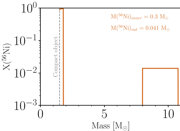
Figure 9. The 56 Ni abundance profile of our preferred model powered by the double-peaked nickel distribution. The stellar surface is at 500 R ⊙ for \sim 11 M ⊙ before explosion (i.e. the outer component is not extended up to the surface). Note that the inner component shows a slightly decline due to presence of other heavy elements such as Si, Ar, or Ca.
