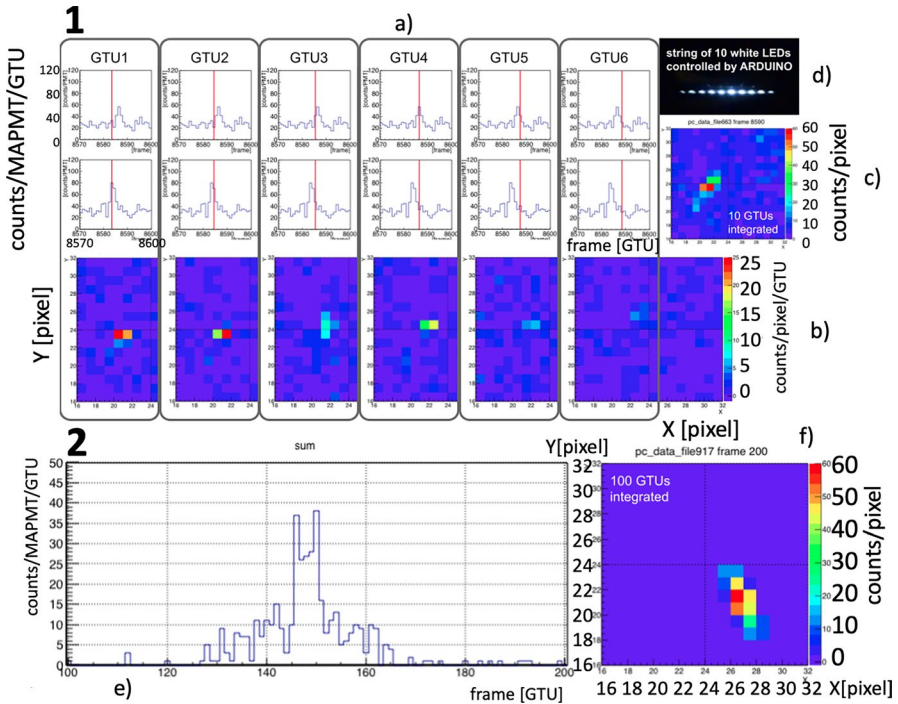
Fig. 19 Reproduction of EAS-like tracks at TurLab in the second phase. Part 1 of the figure shows in 1-a) for 6 GTUs the same light sequence (total counts on 1 MAPMT as a function of 2.5 \mu s GTUs) obtained by illuminating the FoV of the MAPMT with the Arduino-driven LED sequence shown in 1-d). In these 6 panels the total number of counts on one MAPMT is displayed with a red line indicating the specified GTU. The bottom 6 plots (1-b) show the corresponding images at MAPMT level. The 10 GTU integrated image is displayed in 1-c). The average background level is set at \sim 0.5 counts/pixel/GTU. Part 2 of the figure shows for another Arduino-driven event the integrated counts during the event in 2-e) and the full light track in 2-f). In this case no background light is present. Figure adapted from [29]
