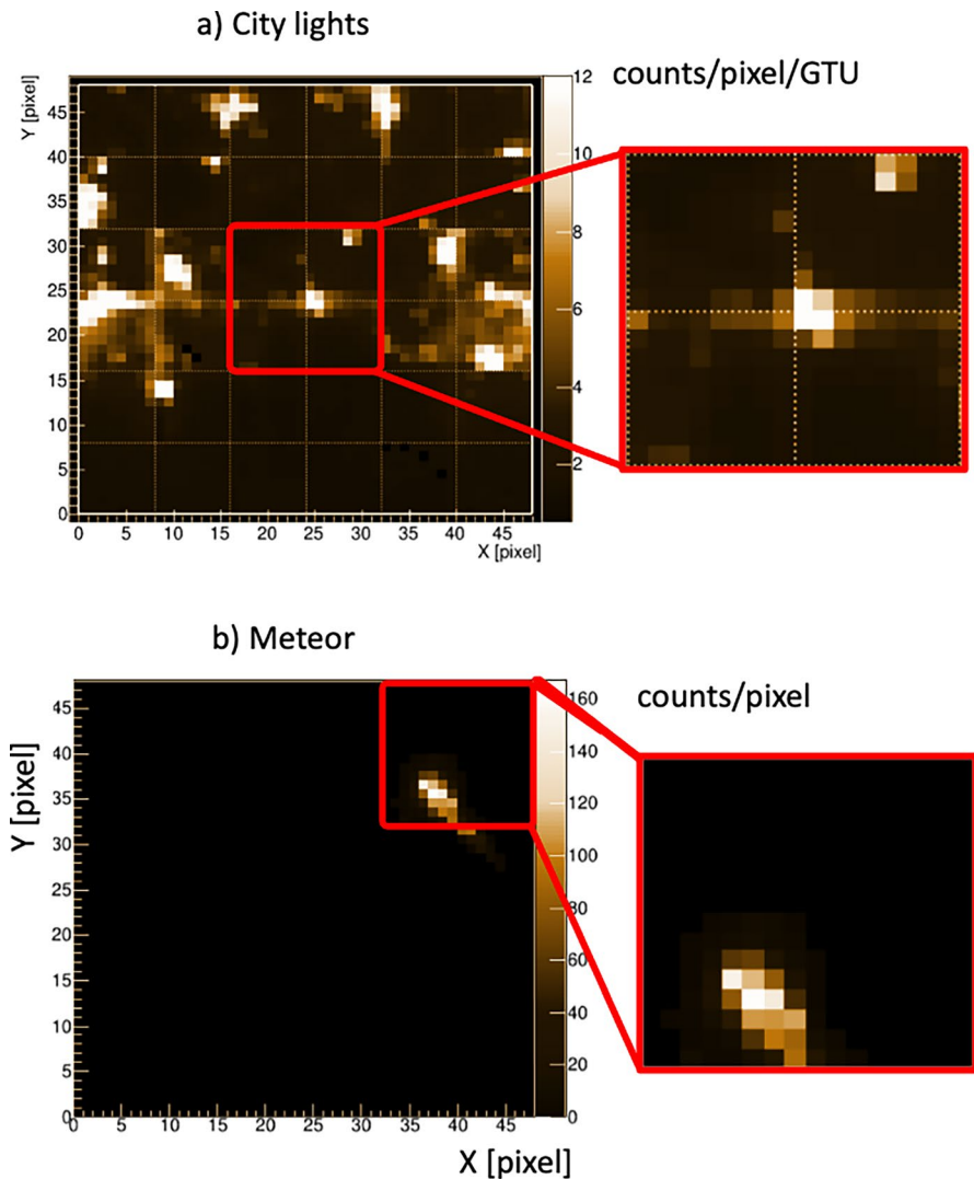
Fig. 17 Images taken by Mini-EUSO (figure adapted from [6]): a) one frame of 320 \mu\text{s} of an urban area on the East coast of India (West Bengal); b) a meteor track integrating over 41 ms time frames; For both plots, a zoom on a single EC scale of 16 \times 16 pixels has been made for a better comparison with EUSO@TurLab images
