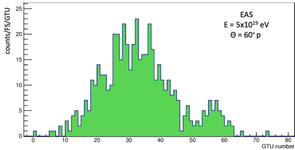
Fig. 1 Light profile of a 5 \times 10^{19} eV proton EAS with zenith angle 60^\circ simulated with the ESAF code [18]. The vertical axis indicates the detected photo-electron counts per data frame (GTU, see text for the definition) on the full Focal Surface of the JEM-EUSO mission
