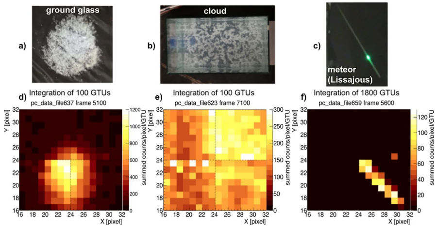
Fig. 15 Top: Examples of UV images obtained by the EC unit (2×2 MAPMTs, phase 2) passing by the various materials during the full tank rotation ( \sim 9 min to be in the range of suitable speeds for Mini-EUSO comparisons, see Table 2): a) city light is emulated by a ground glass illuminated by an LED; b) cloud is emulated using particles suspended in water; c) meteor track is reproduced using an analog oscilloscope. Bottom: the three plots in d) – f) show the corresponding images of a) – c) obtained during each event and integrated during the indicated number of D1 GTUs. It is important to remind that there is a difference in the spectra between the real physical sources and the simulated ones at TurLab. However, what matters is the similarity of the extension of the imaged signal and of the count rates between TurLab and Mini-EUSO setups
