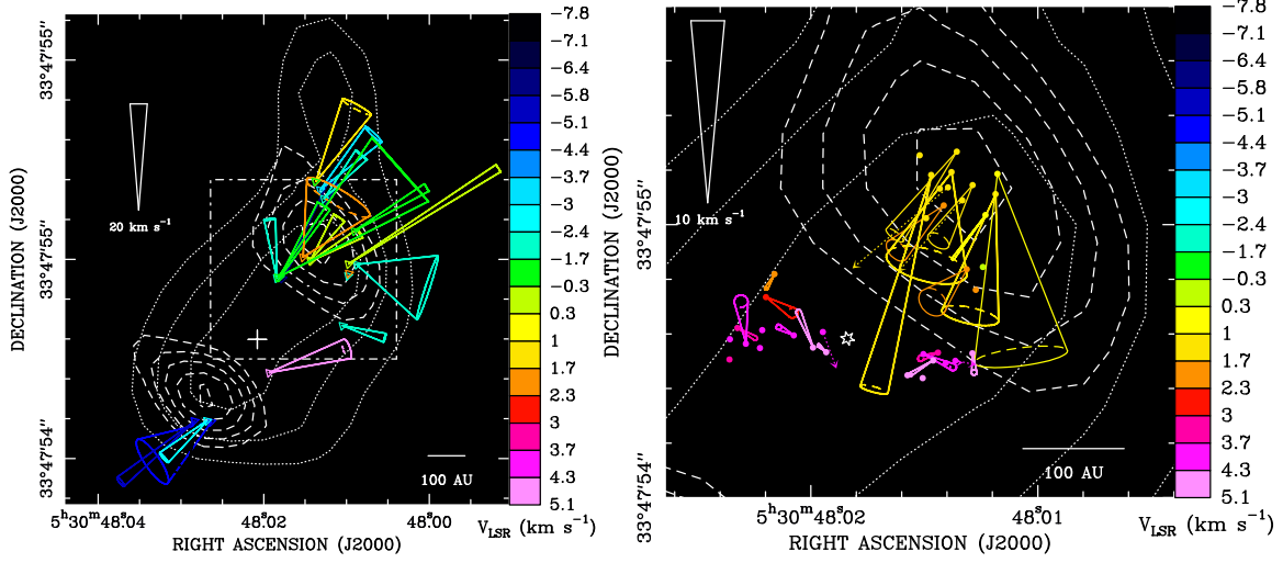
Figure 1: Proper motions of 22 GHz \text{H}_2\text{O} (left panel) and 6.7 GHz \text{CH}_3\text{OH} (right panel) masers in AFGL 5142 MM-1, observed with the VLBA and the EVN, respectively. The rectangle in the left panel shows the area plotted in the right panel. The cones indicate orientation and uncertainties of measured proper motions (the amplitude scale is given in each panel) and colors denote line-of-sight velocities. Contour maps show the VLA 22 GHz (dotted line) and 8.4 GHz (dashed line) continuum. The white star in the right panel identifies the putative location of the protostar.
