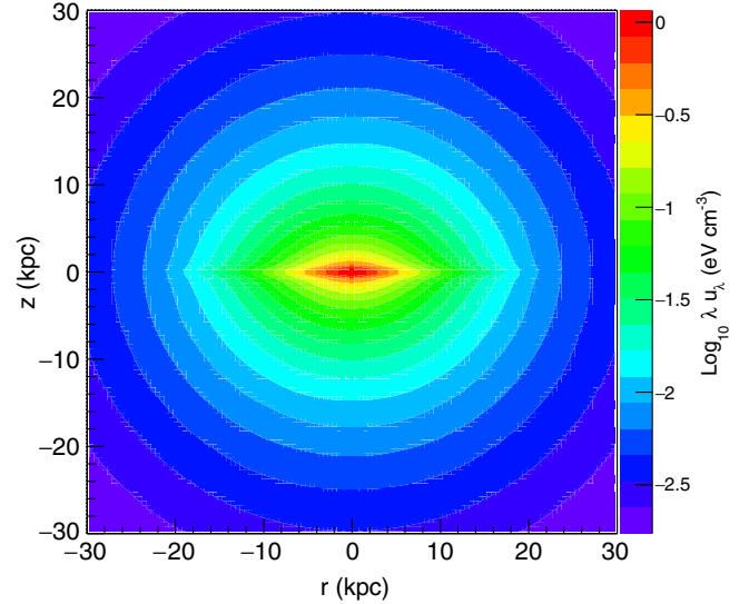
FIG. 6. Space dependence of the angle integrated energy density ( u_\lambda \lambda ) of the infrared radiation for wavelength \lambda = 100 \mu\text{m} , shown as a function of the cylindrical coordinates r and z in the Galaxy system.
