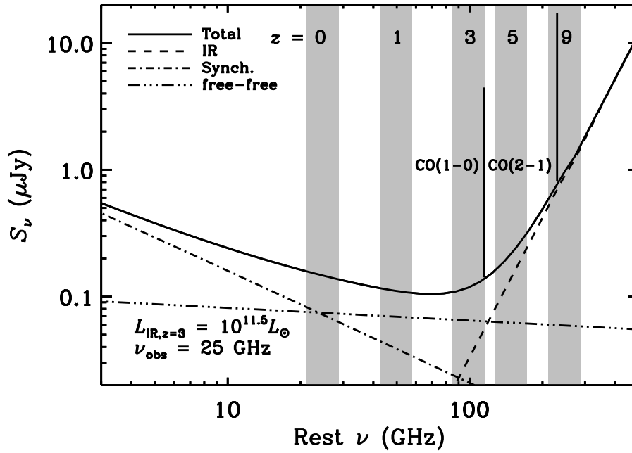
Figure 1: A rest frame model radio-to-infrared galaxy spectrum having an IR (8-1000 \mu m) luminosity of L_{\text{IR}} = 10^{11.5} L_{\odot} at redshift 3. The shaded regions indicate where a 25 GHz observation (see §3), having 30% bandwidth in the observed frame, would redshift for z = 0, 1, 3, 5 , and 9. Individual emission components (free-free, synchrotron, and thermal dust) are shown, indicating that at this frequency range between 30 and 100 GHz (in the rest frame) is most sensitive to free-free emission, making this spectral window extremely robust for accurately measuring the star formation rates of high-redshift galaxies. Additionally shown are CO ( J = 1 \rightarrow 0 ) and CO ( J = 2 \rightarrow 1 ) spectral lines having a line-to-IR flux ratio of M 82 and 1000 km s ^{-1} widths. These lines, which are essential for accurately measuring the molecular gas content of galaxies as they trace the bulk of the cold molecular gas component, are accessible in the redshift range of z = 2.8 - 10.5 over the full 20 – 30 GHz spectral window.
