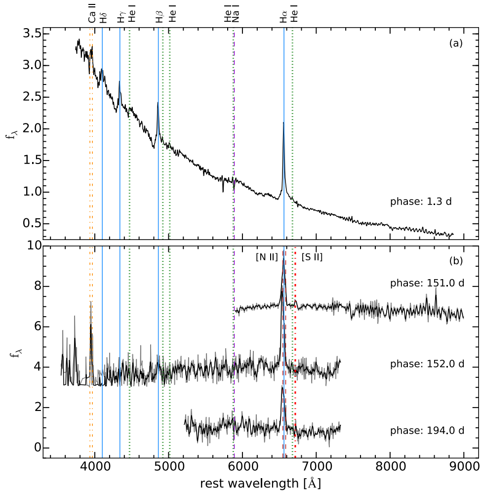
Figure 6. (a) Early-time and (b) late-time optical spectra of SN 2010bt. The late spectra are shown in gray, with a boxcar-smoothed (using a 5 pixel window) version of the spectra overplotted in black. The locations of the most prominent spectral features are indicated by vertical lines. The data used to create this figure are available.
