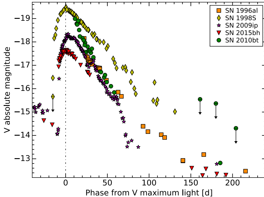
Figure 3. Absolute V light curve of SN 2010bt (circles), along with those of the SNe IIn SN 1996al (squares) and SN 1998S (diamonds) and the controversial transients SN 2009ip (stars) and SN 2015bh (inverted triangles). Upper limits are indicated by symbols with arrows. The dot-dashed vertical line indicates the V -band maximum light of SN 2010bt. Ages are relative to V maximum light (we have assumed V maximum date = discovery date – 10 days, for SN 2010bt).
