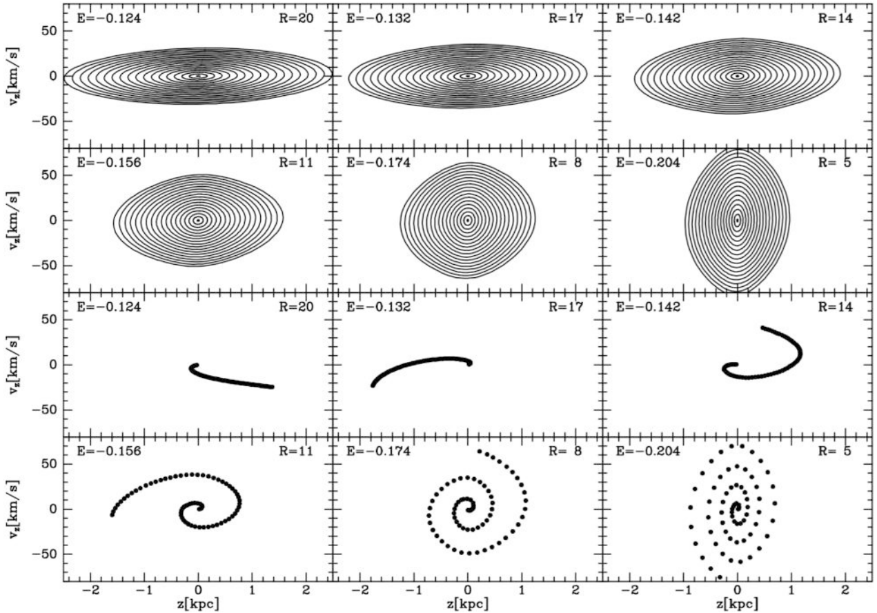
Figure 20. The top six panels show surfaces of section in the vertical phase plane (z, V_z) at six different radii ( R = 20, 17, 14, 11, 8 , and 5 kpc) which are chosen to match the radial extent of our new disc simulations and the Gaia /GALAH study. The panels were computed with the AGAMA software package (Vasiliev 2018) adopting the Galactic potential from Piffl et al. (2014). The amplitude of the outer ellipse and the phase spiral at R = 8 kpc are chosen to match the Gaia data. In every panel, the outermost ellipse has the same area ( =2\pi J_z ) and the orbital energies E are indicated. The J_z values for each concentric ellipse moving outwards are: 0.008, 0.20, 0.65, 1.35, 2.31, 3.52, 4.99, 6.71, 8.69, 10.93, 13.42, 16.17, 19.17, 22.43, 25.94, 29.71, 33.73, and 38.01 \text{kpc km s}^{-1} . In the outer disc, the ellipses elongate in z because stars travel farther and slower in the weaker disc potential. All orbits have radial action J_R = 0.01 \text{ kpc}^2 \text{ Myr}^{-1} = 9.78 \text{ kpc km s}^{-1} and J_\phi for the circular orbit at the quoted radius. The bottom six panels coincide with the panels above indicated by the total energies; these reveal the impact of phase wrapping after 250 Myr where all points are initially lined up along the z < 0, V_z = 0 axis. Across the inner disc, the stronger disc gravity leads to faster vertical oscillations which result in faster phase wrapping.
