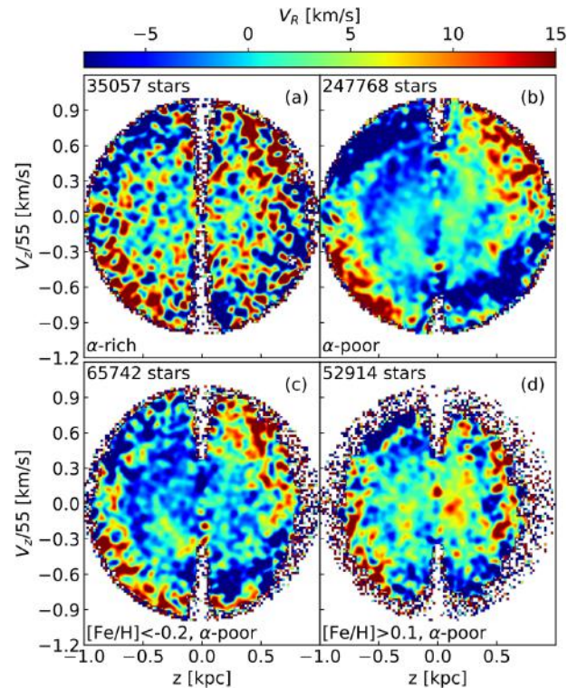
Figure 18. Map of median V_R in (z, V_z) plane for stars in the solar neighbourhood using data from GALAH and Gaia DR2. The sample definitions are the same as in Fig. 10.
