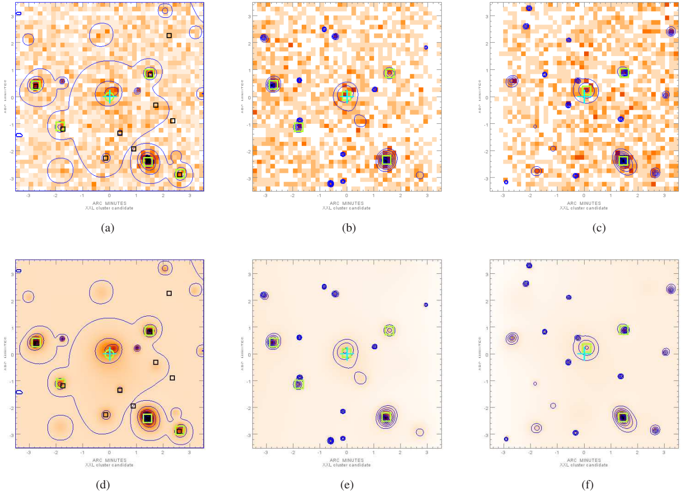
Fig. 8. Using tiles allows us to recover a cluster that would be missed using separate pointings. In all images a green circle indicates an extended source (C1 or C2 detection) and a green square a source that is significant (PNT_DET_STAT > 15) but which cannot be securely identified as point-like or extended; the cyan cross shows the position of the recovered cluster and the black squares in the left panels the position of the input AGNs; X-ray contours are also shown. Panel a: combined photon image. Panel b: photon image of one of the pointings. Panel c: photon image of the other pointing. Panel d: combined wavelet image. Panel e: wavelet image of one of the pointings. Panel f: wavelet image of the other pointing.
