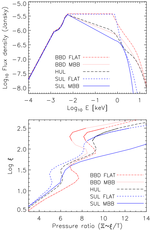
Figure 5. SED (top) and stability curves (bottom) of ULX NGC 1313 X-1 calculated for different states (soft, SUL; bright-broadened-disc, BBD; and hard ultraluminous, HUL; see Table A1). The solid intervals in the bottom plot indicate the RGS best-fitting wind solution ( 0.2c ) obtained in Pinto et al. (2016). Two different continuum models for the BBD and SUL SEDs are tested here (see Section 3.4). During the brightest BBD state, the gas might move towards an unstable branch.
