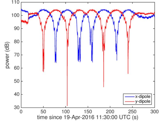
Figure 6. Output power of the x- and y-dipoles of the central LBA element measured during the spin flight.
