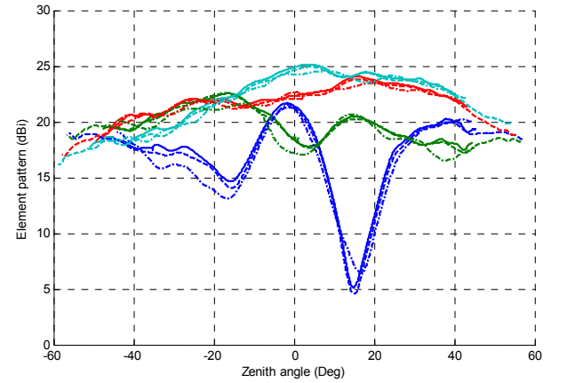
Figure 7. Measured LBA embedded patterns at 57 MHz: Central Element (blue), Element #2 (green), Element #26 (red), Element #42 (cyan). Elements with higher label number are further from the center.
