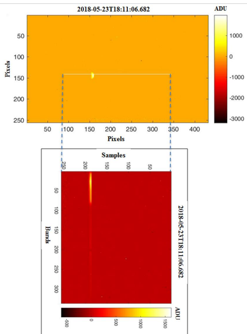
Figure 10: Ganymede observation, during PJ13, acquired by both the JIRAM Imager and Spectrometer. In the image are shown the simultaneous acquisitions of the Imager (top) and Spectrometer (down). Top: the M filter
