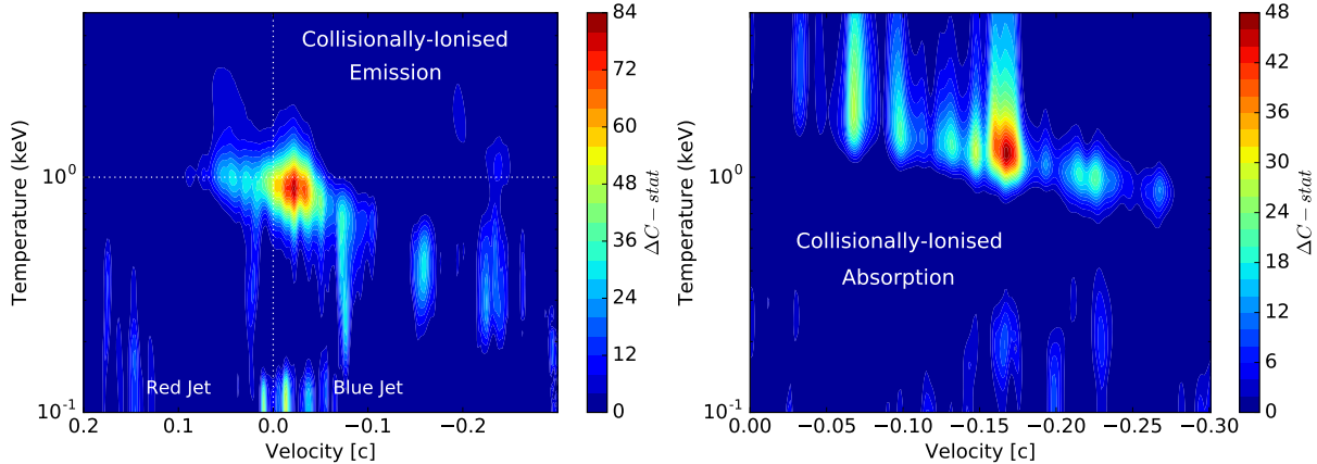
Figure 9. Multi-dimensional scans of collisional-ionisation emission (left panel) and absorption models (right panel) for NGC 247 ULX-1 time-averaged EPIC+RGS spectra. The X-axis shows the line-of-sight velocity (negative means blueshift, i.e. motion towards the observer). The color is coded according to the \Delta C fit improvement to the spectral continuum model.
