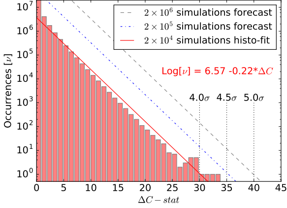
Figure A4. Histogram and corresponding power-law fit of the 20k Monte Carlo simulations of NGC 247 ULX-1 and forecast for 200 000 and 2 million simulations.
