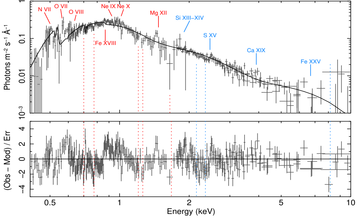
Figure 6. Top panel: time-averaged XMM-Newton RGS (0.33–2 keV) and EPIC MOS 1,2-pn (1.77–10 keV) spectra. Overlaid is the baseline 3-blackbody continuum model (solid black line, see Table 2). The bottom panel shows the residuals calculated with respect to the continuum model. The rest-frame energies of the most common strong transitions in the X-ray band (red for RGS band and blue for EPIC) and the absorption features (dotted lines) are also shown. All spectra were rebinned for displaying purposes.
