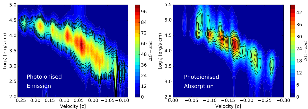
Figure 10. Scans of photoionisation emission (left) and absorption (right) models for the time-averaged EPIC and RGS spectra. Labels are same as in Fig. 9. The black contours refer to the (2.0, 2.5, ... 4.5, 5.0) \sigma confidence levels estimated by Monte Carlo simulations.
