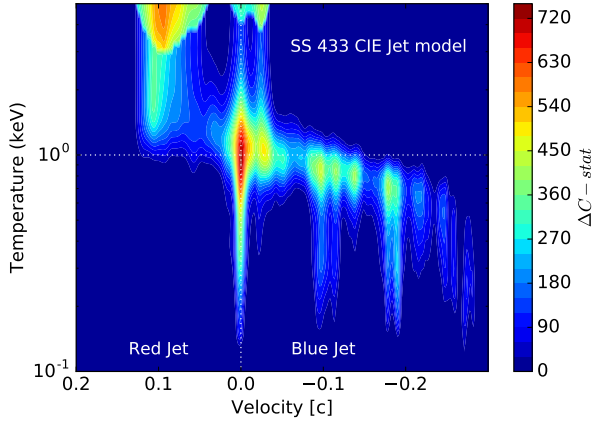
Figure A2. Multi-dimensional scan of collisional-ionisation emission model for the SS 433 RGS spectrum. The X-axis shows the line-of-sight velocity. Labels are same as in Fig. 9.
