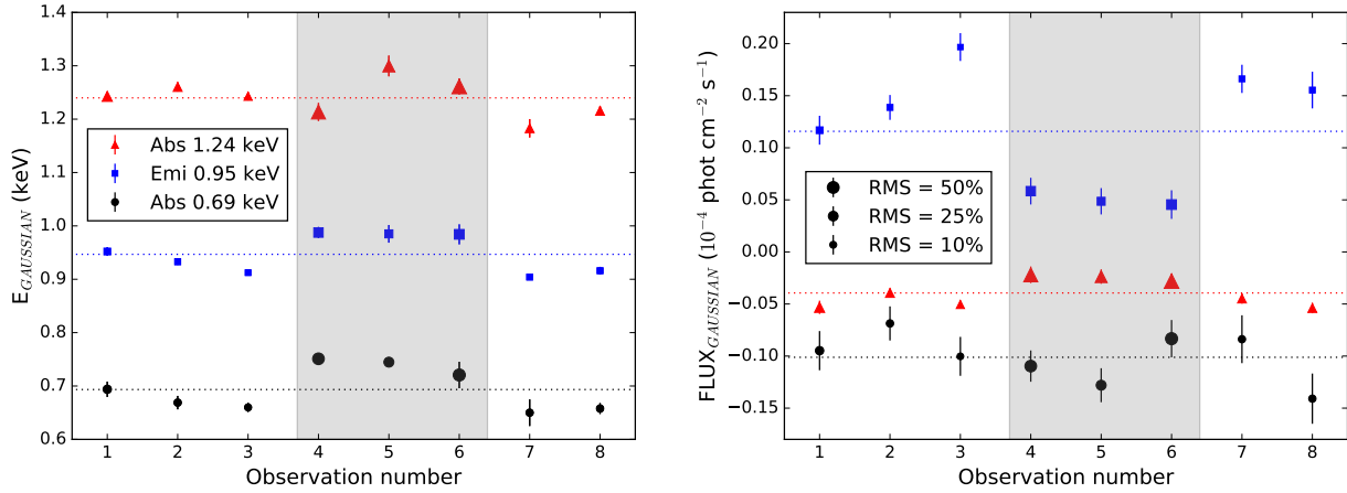
Figure 4. Evolution of the XMM-Newton EPIC spectral residuals around 1 keV. The left and the right panels show the energy centroid and normalisation of the Gaussian lines used to fit the three main (unresolved) spectral residuals, respectively. The shaded grey areas highlight the observations of high spectral variability and dipping. ‘Abs’ and ‘Emi’ refer to absorption and emission features, respectively.
