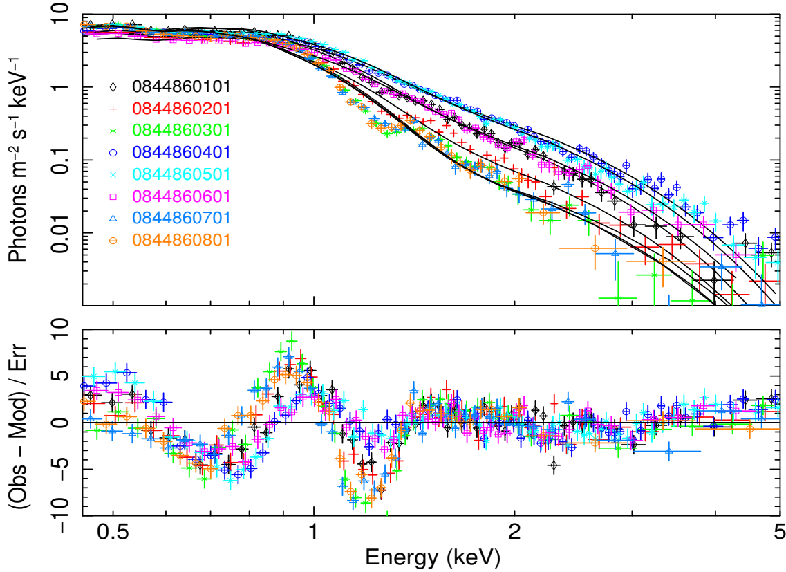
Figure 3. XMM-Newton EPIC-pn spectra of NGC 247 ULX-1. The top panel shows the pn spectra of the individual observations with overlaid the 2-blackbody continuum models. The bottom panel shows the corresponding residuals. Both the emission feature below 1 keV and the absorption feature above 1 keV vary in centroid and strength according to the continuum flux and shape. This is qualitatively similar to the intermediate-hard source NGC 1313 ULX-1 and the soft source NGC 55 ULX-1 (Middleton et al. 2015b; Pinto et al. 2017).
