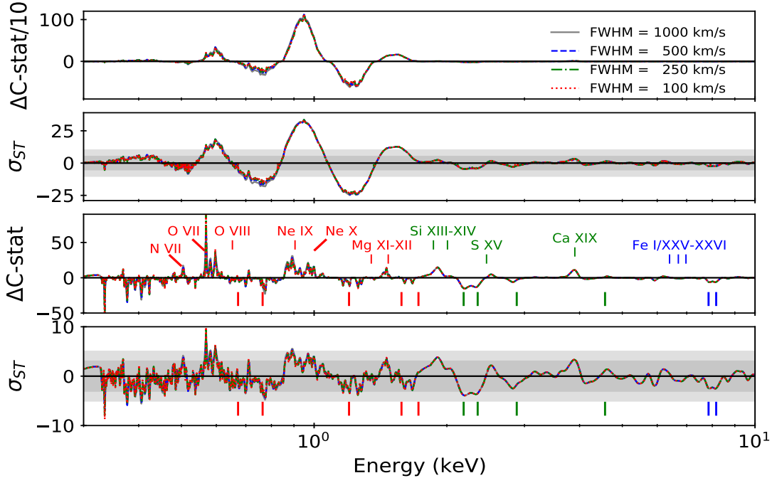
Figure 8. Gaussian line scan performed on the time-averaged XMM- Newton EPIC and RGS spectra of NGC 247 ULX-1. The top panels show the case when the EPIC spectra are used throughout the whole 0.3–10 keV band, while the bottom two panels show the results obtained with RGS between 0.33–2 keV and EPIC-pn from 1.77–10 keV (see also Fig. 6). The results for four different line widths are shown. No remarkable difference is observed among the adopted widths. The single-trial line significance (“ \sigma_{ST} ”) is calculated as square root of the \Delta C times the sign of the Gaussian normalisation (positive/negative for emission/absorption lines). Labels are red for RGS, green for strong EPIC features and blue for the faint Fe K. The grey shaded areas show the 3 and 5 \sigma_{ST} limits for individual lines.
