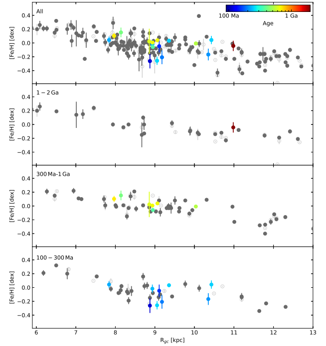
Fig. 11. Run of [\text{Fe}/\text{H}] versus R_{\text{gc}} for the studied clusters, colour-coded as a function of their age. Dark and light grey points are the clusters in Zhang et al. (2021) and Spina et al. (2021), respectively, which are plotted for comparison. Top panel: whole sample, while the remaining panels show three different age ranges.
