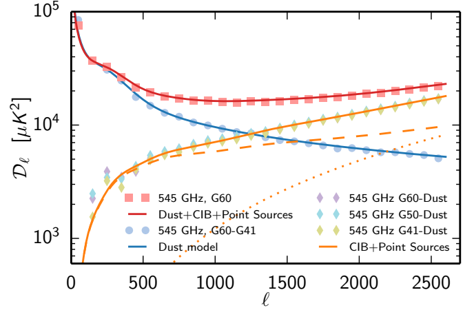
Fig. 19. Dust model at 545 GHz. The dust template is based on the G60–G41 mask difference of the 545 GHz half-mission cross-spectrum (blue line and circles, rescaled to the dust level in mask G60). Coloured diamonds display the difference between this model (rescaled in each case) and the cross half-mission spectra in the G41, G50, and G60 masks. The residuals are all in good agreement (less so at low \ell , because of sample variance) and are well described by the CIB+point source prediction (orange line). Individual CIB and point sources contributions are shown as dashed and dotted orange lines. The red line is the sum of the dust model, CIB, and point sources for the G60 mask, and is in excellent agreement with the 545 GHz cross half-mission spectrum in G60 (red squares). In all cases, the spectra were computed by using different Galactic masks supplemented by the single combination of the 100 GHz, 143 GHz, and 217 GHz point sources, extended objects and CO masks.
