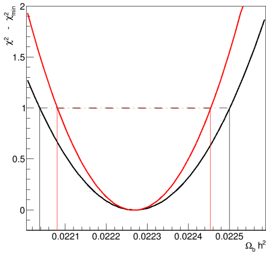
Fig. E.7. Likelihood (specifically \chi^2 - \chi_{\min}^2 ) profile of \Omega_b h^2 within the \Lambda CDM model for Plik. In black is shown the full profile-likelihood fit (to derive the full error of Table E.4) and in red the profile-likelihood fit when the nuisance are fixed to the values obtained when maximizing the likelihood function (to derive the “sensitivity related” error of Table E.4).
