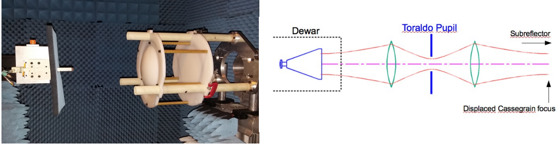
Fig. 3 Left panel. Laboratory setup showing the two-lens collimator, illuminated by a K-band corrugated feed horn. The focus fields are sampled with a an open waveguide. Right panel. Gaussian-beam propagation in the collimator.
