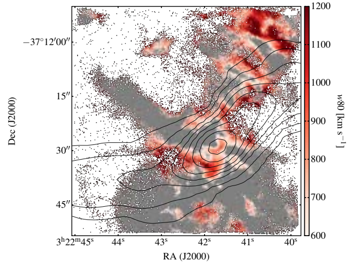
Fig. 13. Map of the w80 of the total [NII] \lambda 6583 line. Values above 600 \text{ km s}^{-1} may indicate the presence of outflowing gas, and are shown in colour scale. The radio jets are shown by black contours.
