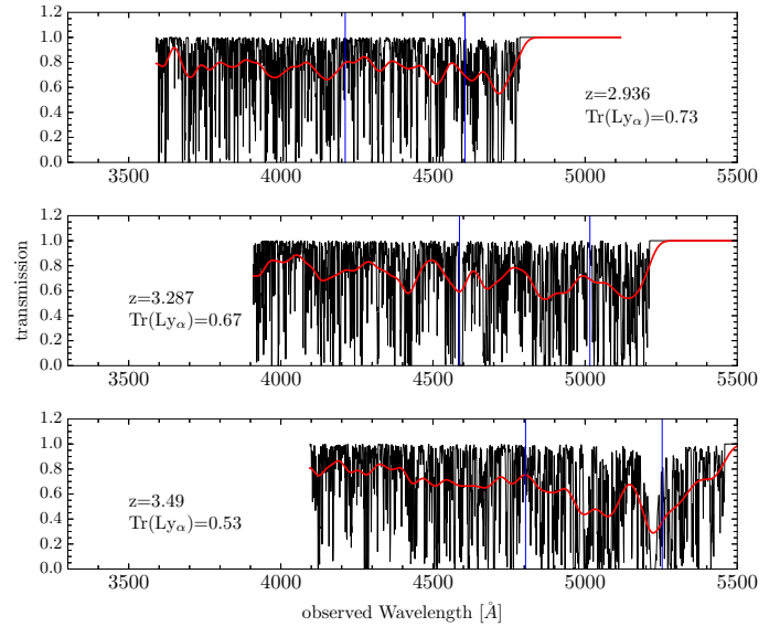
Fig. 5. Three examples of \text{Ly}\alpha skewers at z = 2.936 , z = 3.287 , and z = 3.49 . In each plot, the black spectrum represents the high spectral resolution BOSS DR11 mock IGM transmission, while the same spectrum in red is degraded to the VUDS lower resolution. The blue lines in each panel represent the wavelength interval where the \text{Ly}\alpha transmission is estimated (1070–1170 Å).
