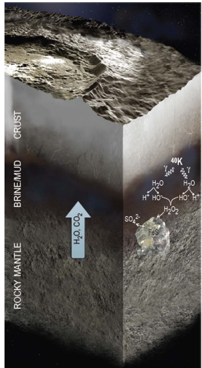
Figure 4. Summary of processes that may alter the chemical properties of a deep ocean over time: loss of volatiles from the mantle upon thermal metamorphism and radiolysis. The Occator impact itself could introduce exogenic material in the crust. Based on Altair et al. (2018); background rendering from Raoul Ranao.
