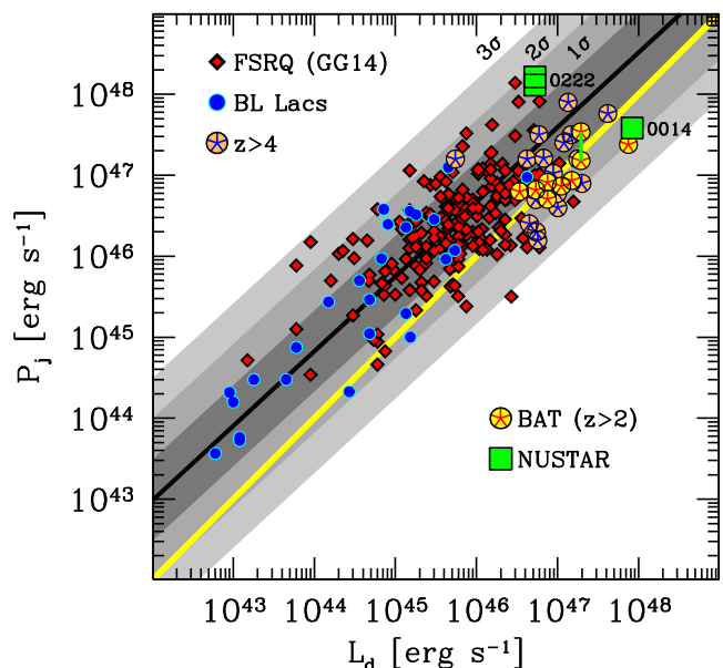
Figure 4. Total jet power as a function of accretion disc luminosity in blazars. Red (outlined in black) diamonds and blue filled circles are, respectively, FSRQs and BL Lacs from Ghisellini et al. (2014). Circled asterisks are high-redshift, non- \gamma -ray detected blazars: pink filled circles with blue asterisks are all the known z > 4 blazars (see Ghisellini et al. 2015), yellow filled circles with red asterisks are the z > 2 blazars detected by Swift /BAT. Green filled squares are S5 0014+318 and B0222+185 (both states) as labelled, observed by NuSTAR for this work. Note that the latter are the two blazars with the most luminous accretion disc (S5 0014+318) and the most powerful jet (B0222+185). The black line and grey stripes are the best-fitting relation of \gamma -ray detected blazars from Ghisellini et al. (2014), along with the 1\sigma , 2\sigma and 3\sigma dispersions. The yellow line is the one-to-one correlation. S5 0836+710 underwent a prominent \gamma -ray flare, and therefore it has been plotted with the jet powers of both its average and flaring states. The two states are connected with a green line. This suggests that part of the spread could be due to different states of the single sources, along with flaring episodes. The jet power is calculated as the sum of the different components listed in Table 3. Note that the very powerful blazars we added to the original sample by Ghisellini et al. (2014) are located within 2\sigma from the \gamma -ray detected jet–accretion relation. This means that also in the most powerful sources the jet power correlates with accretion luminosity, but it is larger than the accretion power, leading to an important role of black hole spin in jet launching.
