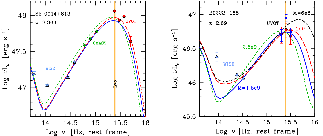
Figure 2. IR-optical-UV SEDs of S5 0014+813 and B0222+185, along with models used to derive L_d and M_{BH} . In both panels, the yellow vertical line highlight the Ly \alpha line position. At frequencies larger than this line, the Swift /uvot data points have been corrected for the absorption by intervening clouds. The cloud distribution, though, is random and strongly dependent on the line-of-sight. Hence the absorption correction is only statistical, with little reliability on single sources. We do not consider this wavelength range for our modelling. Left-hand panel: S5 0014+815 IR-optical-UV SED. The red circles are new Swift /uvot data. Green diamonds are 2MASS and blue triangles are WISE data points. The solid blue line corresponds to our best model, with M_{BH} = 7.5 \times 10^9 M_\odot and L_d = 0.85 L_{Edd} = 8.3 \times 10^{47} \text{ erg s}^{-1} . The green short dashed line shows a model with M_{BH} = 10^{10} M_\odot and L_d = 0.7 L_{Edd} = 9.1 \times 10^{47} \text{ erg s}^{-1} , while the red long dashed line with M_{BH} = 7 \times 10^9 M_\odot and L_d = L_{Edd} = 9.1 \times 10^{47} \text{ erg s}^{-1} . The last two represent the ‘confidence range’ of M_{BH} and L_d . Right-hand panel: B0222+183 IR-optical-UV SED. Red circles are Swift /uvot data from the January observation, blue squares from the December observation. Blue triangles are archival WISE data points. The solid blue line is the best model, with M_{BH} = 1.5 \times 10^9 M_\odot and L_d = 0.27 L_{Edd} = 5.3 \times 10^{46} \text{ erg s}^{-1} . The red long dashed line corresponds to M_{BH} = 1 \times 10^9 M_\odot and L_d = 0.42 L_{Edd} = 5.5 \times 10^{46} \text{ erg s}^{-1} , while the green short dashed to M_{BH} = 2.5 \times 10^9 M_\odot and L_d = 0.17 L_{Edd} = 5.5 \times 10^{46} \text{ erg s}^{-1} . The black dot-dashed line represents instead a tentative model obtained by trying to fit the uvot December data at \nu = 10^{15.4} \text{ Hz} . The last two represent the ‘confidence range’ of M_{BH} and L_d .
