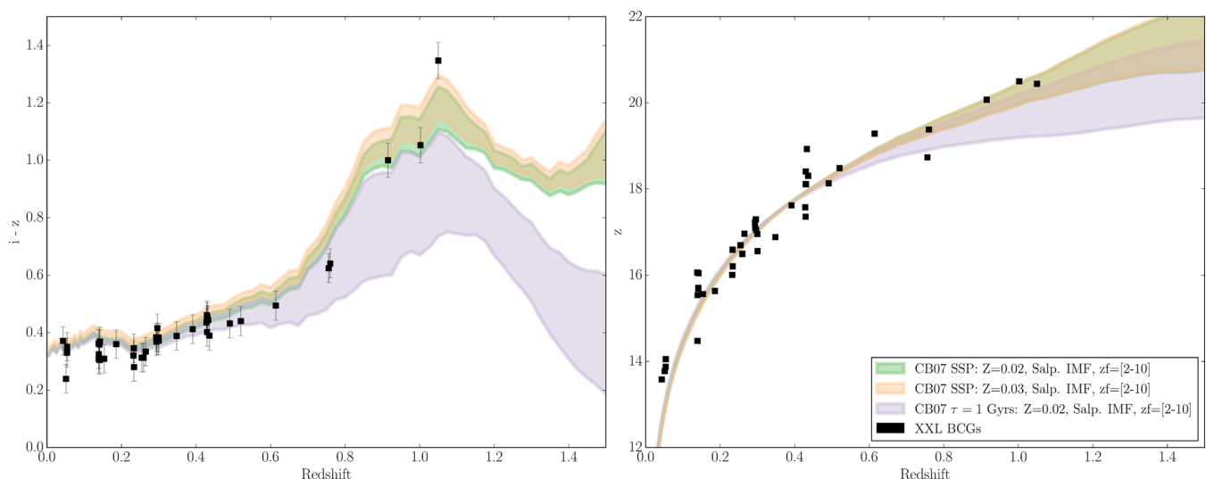
Figure 5. Colour (left) and z -band magnitude (right) evolution of the XXL-100-GC North subsample. The green band represents the evolution of the best-fitting model for z_f between 2 and 10 with solar metallicity and Salpeter IMF. The red band is the same model with 1.5 \times Z_{\odot} and the blue band is a model with solar metallicity and \tau = 1 Gyr. The black squares represent XXL-100-GC North BCGs. Both panels use the same legend.
