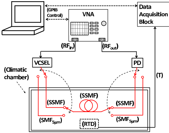
Fig. 4. Functional scheme of the experimental setup.
