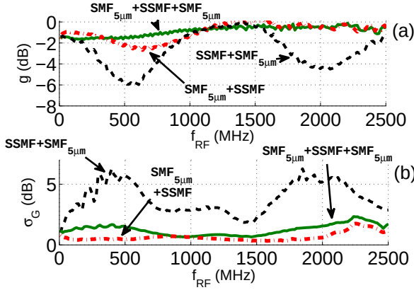
Fig. 6. Behaviors of g (a) and \sigma_G (b) versus frequency of three VCSEL based transmission links utilizing 300 m of SSMF, respectively with a patchcord of SMF_{5\mu m} at the beginning, at the end, and both at the beginning and at the end of the SSMF span. As in Fig. 5 (b), the curves reported in (b) are also representative of the standard deviation \sigma_{NF} of the noise figure NF of the links considered.
