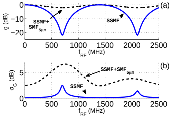
Fig. 1. Comparison of simulated results for a transmission link with SSMF length L_1 = 300 m in case of presence and in case of absence of SMF_{5\mu m} patch between SSMF and PD. The bandwidth improvement due to the SMF_{5\mu m} employment can be noticed in (a) while the increase of the standard deviation \sigma_G of the fluctuations of G due to modal noise is shown in (b). The parameters values utilized in the simulation program are: m_I = 0.375 , A_1^2 = 0.55 , A_2^2 = 0.45 , a_{11}^2 = 0.9 , a_{12}^2 = 0.065 , b_{11} = 0.985 , b_{22} = 0.985 , b_{12} = 0.015 .
