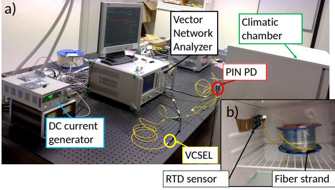
Fig. 3. Experimental setup utilized evidencing its portions placed (a) outside and (b) inside the climatic chamber.
