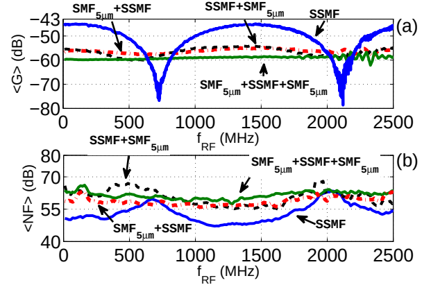
Fig. 7. Behaviors of (a) the average RF gain \langle G \rangle for L_1 = 300 m and (b) the noise figure NF , in the four configurations of VCSEL-based transmission links considered in the present work.
