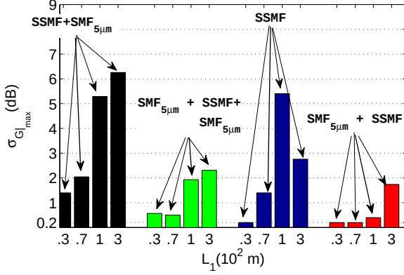
Fig. 8. Behaviors of \sigma_G|_{max} for links of different length L_1 in the four configurations of VCSEL-based transmission links considered in the present work.
