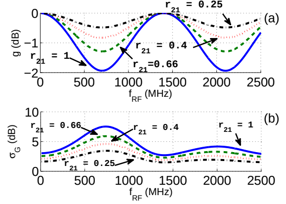
Fig. 2. Behavior of g (a) and \sigma_G (b) as a function of the RF modulating frequency as function of the parameter r_{21} = (A_2/A_1)^2 . A reduction in both \Delta g and \sigma_G can be noticed due to the reduction of A_2 with respect to A_1 . The transmission link considered is the one with SSMF length L_1 = 300 m in case of presence of SMF_{5\mu m} patch between SSMF and PD.
