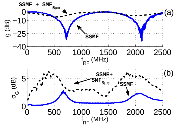
Fig. 5. Behaviors of g (a) and \sigma_G (b) versus frequency of two VCSEL based transmission links utilizing 300 m of SSMF, respectively with and without SMF_{5\mu m} at the end of the SSMF span. The curves reported in (b) coincide with the curves representing the standard deviation \sigma_{NF} of the noise figure NF of the links considered.
