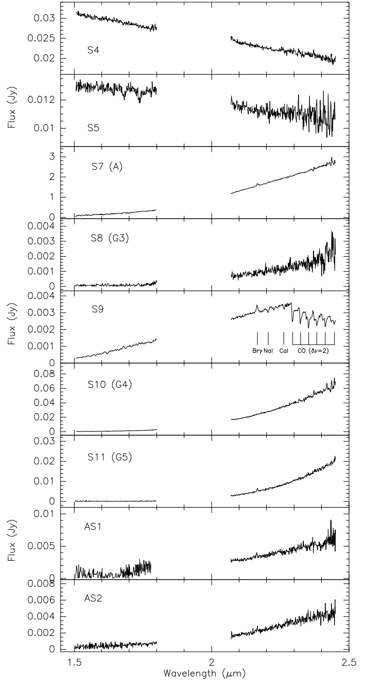
Fig. 2. Near infrared HK spectra of objects in the region associated with IRAS 18511. The gap in the spectra between 1.8 and 2.1\,\mu\text{m} is due to atmospheric absorption.
