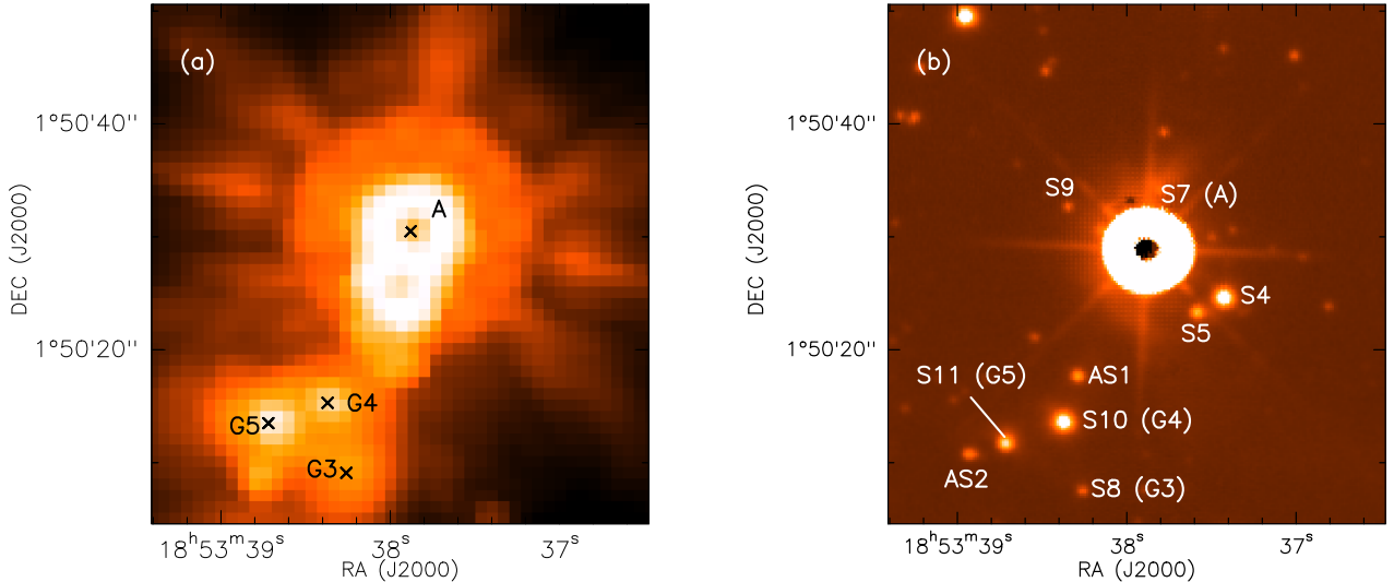
Fig. 1. a) Spitzer -GLIMPSE 8 \mu\text{m} and b) UKDISS – GPS K -band image of IRAS 18511 region. a) The mid-infrared sources 18511-A (S7) as well as young stellar objects G3–G5 are marked. The sources for which near-infrared spectroscopy have been carried out are shown in b) .
