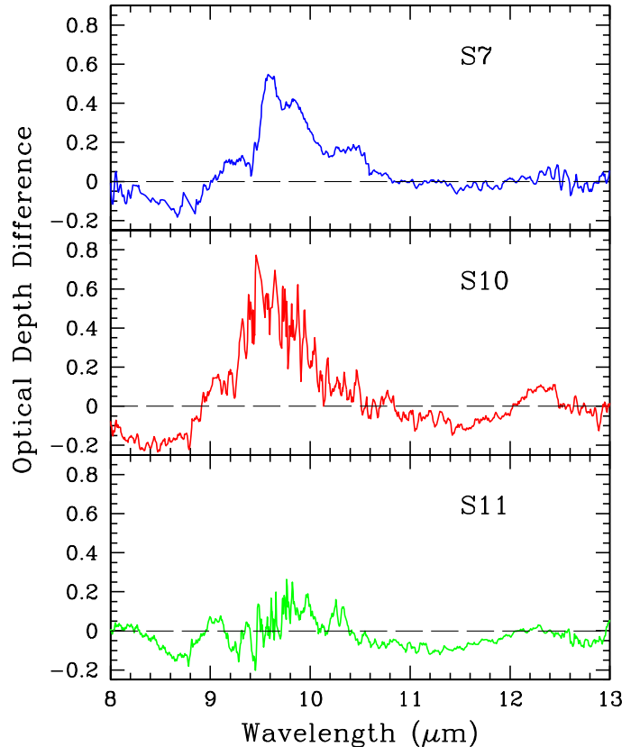
Fig. 10. Difference spectra of the silicate optical depth profiles between the observed and Galactic centre (GC) of the sources S7, S10 and S11.
