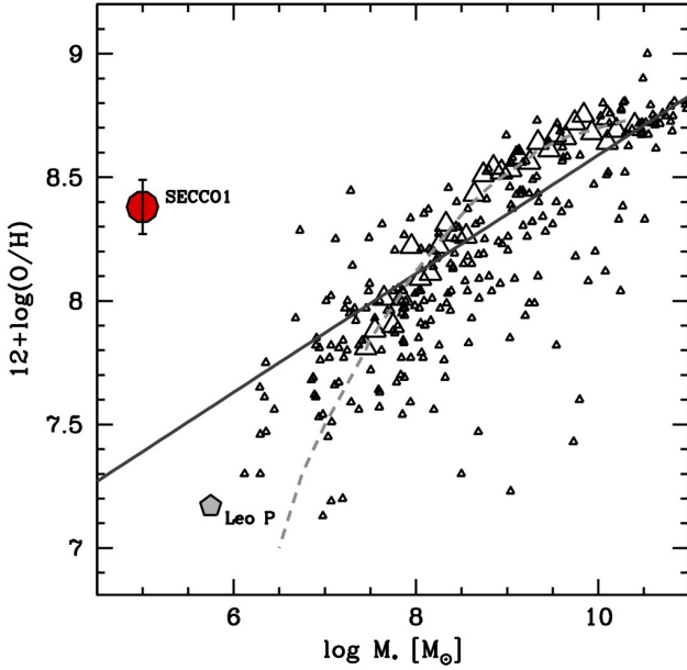
Figure 10. SECCO 1 as a whole into the stellar mass - metallicity relation. Small triangles are the z \approx 0 sample of Hunt et al. (2016), large triangles are from Andrews & Martini (2013), the light grey long-dashed curve is the best-fit to the same data (from direct-method oxygen abundance estimates) extrapolated to low masses, from the same source. The dark grey continuous line is the stellar mass - metallicity relation from planetary nebulae by Gonçalves et al. (2014). SECCO 1 is represented as a large red filled circle.
