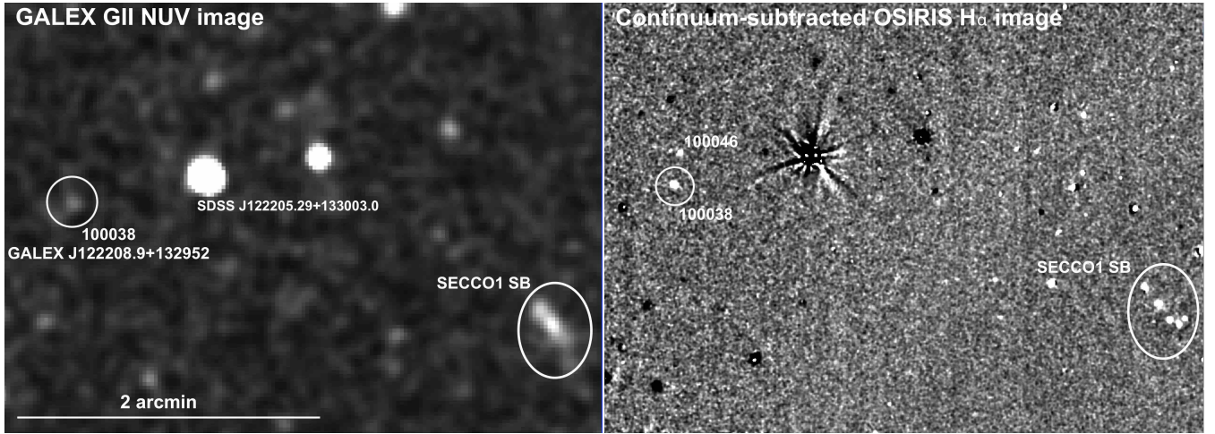
Figure 8. The newly identified candidate H \alpha emitter in the surroundings of SECCO 1. Left panel: GALEX NUV image (with a Gaussian smoothing of 3 px size applied) with the source (100038 / GALEX J122208.9+132952) labeled. A nearby bright star is also identified for reference, as well as SECCO 1 SB. Right panel: continuum-subtracted H \alpha image from our GTC-OSIRIS observations. In addition to 100038 and SB, here we labelled the possible companion source 100046. Note that there are sources (outside SB) that have a significant residual in the H \alpha image but have no counterpart at all in GALEX (and vice versa). In both images North is up and East to the left.
