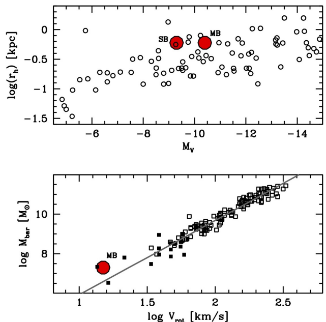
Figure 9. Upper panel: SECCO 1 MB and SB (large red filled circles) in the integrated absolute V magnitude vs. \log of the half-light radius diagram. Small empty circles are dwarf galaxies in the Local Group from McConnachie (2012) . As a proxy for the half-light radius for MB and SB we adopted half of the radial size reported (and defined) in Tab. 1. Lower panel: baryonic Tully-Fisher relation. Open squares are from Lelli et al. (2016) and filled squares from Iorio et al. (2017) ; the grey line is the best-fit for the accurate distances sample by Lelli et al. (2016) . The baryonic mass of SECCO 1 MB (large red filled circle) has been computed by summing the H I mass corrected for the contribution of helium to the total gas mass according to Lelli et al. (2016) ; the rotation velocity is from A15 that provide an estimate of this quantity only for MB.
