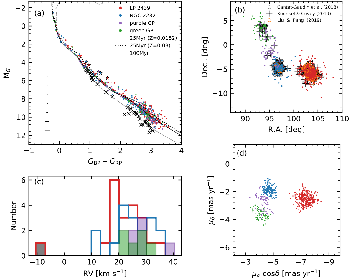
Figure 2. General properties of identified member candidates. (a) The color magnitude diagram of Gaia DR2 absolute magnitude M_G (adopting Gaia DR2 parallax) for candidate stars identified by STARGO. Red and blue dots are candidate members of LP 2439 and NGC 2232. The purple and green dots indicate candidates of the purple and green groups in Figure 1 (c). Crosses indicate field contaminants that are excluded from further investigation. The PARSEC isochrones of 25 Myr and 100 Myr are overplotted as the black solid curve and grey dashed curve, with E(B - V) = 0.07 mag (Lyra et al. 2006) corrected and solar metallicity assumed. The black dotted curve is the PARSEC isochrone of 25 Myr adopting the same reddening but a supersolar metallicity of [\text{Fe}/\text{H}] = 0.32 (Monroe & Pilachowski 2010). The asterisks indicate binary candidates. The red outlined grey shaded asterisk corresponds to the grey shaded bin in panel (c). Uncertainties of colors are indicated with horizontal error bars. The typical G magnitude error is 0.002 mag. (b) The spatial distribution of member candidates after CMD cleaning. The symbols and colors of member candidates are identical to those in panel (a). Members cross-matched with previous catalogs: Cantat-Gaudin et al. (2018), black open circles; Kounkel & Covey (2019), black crosses; Liu & Pang (2019), orange open circles. (c) is the RV histograms for LP 2439 (red), NGC 2232 (blue), the purple group and the green group. (d) shows the proper motion vector plot with colors and symbols the same as panel (a) for member candidates.
