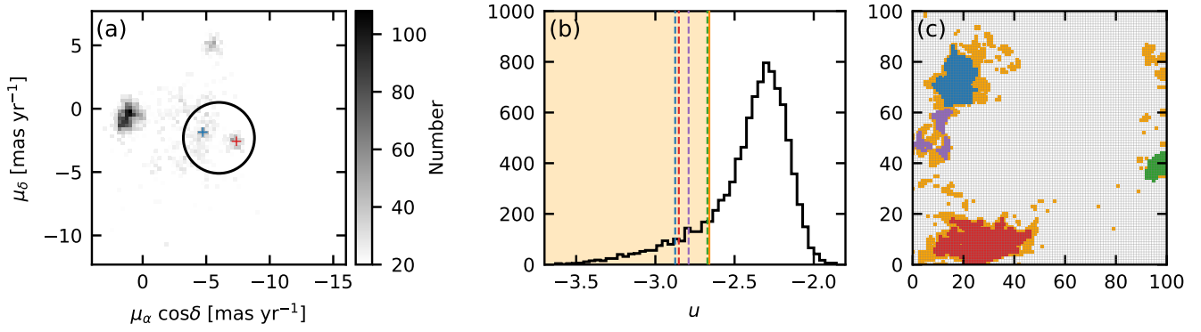
Figure 1. (a) the 2D density map of the proper motion vectors for the regions around NGC 2232 and LP 2439 in Sample I. The blue and red crosses indicate the over-densities generated by NGC 2232 and LP 2439, respectively. Each bin is smoothed by neighboring 8 bins and here only bins with a number count > 3\sigma are shown, where \sigma is the standard deviation of all bins. The color bar indicates the number count in each bin. (b) Histogram of the distribution of u . The orange solid line shows the position u_{\text{peak}} - 3\sigma . The left tail with u < u_{\text{peak}} - 3\sigma is highlighted in orange, corresponding to the orange patches in panel (c). The blue, red, purple, and green dashed lines denote the threshold values of u . Values smaller than this threshold produce the 5% contamination rate among identified candidates for the red, blue, purple and green patches in SOM (panel (c)). (c) 2D 100 \times 100 neural map resulting from SOM, the neurons with u smaller than the threshold values (blue, red, purple and green dashed lines in panel (b)) of the 5% contamination rate are colored as blue, red, purple and green. The two dominant neuron groups are traced with blue (NGC 2232) and red (LP 2439).
