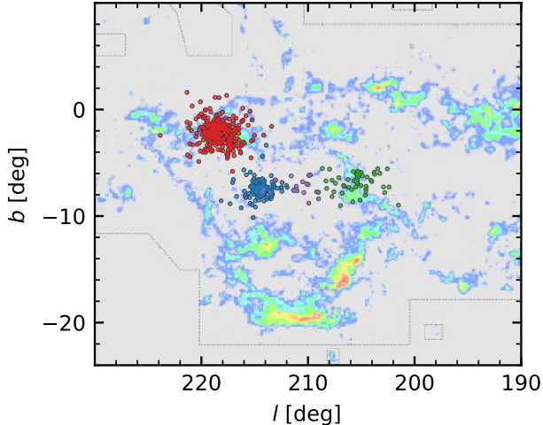
Figure 3. CO emission map obtained from Dame et al. (2001) in the region where member candidates reside. The red dots are candidate members of LP 2439, and the blue dots are candidate members of NGC 2232. The purple and green dots represent the purple and green groups, respectively.
