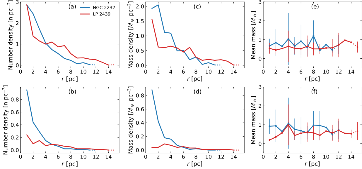
Figure 5. The number density, mass density, and mean mass distributions along cluster-centric distance r for NGC 2232 (blue curves) and LP 2439 (red curves). (a): Surface number density profile; (b): volume number density profile. (c): surface mass density profile; (d): volume mass density profile. (e): distribution of mean stellar mass in each surface annulus; (f): distribution of mean stellar mass in each volume annulus. The error bar is the standard deviation of the stellar mass in each annulus. The values for the outermost data points (at r = 12 pc for NGC 2232 and at r = 15 pc for LP 2439) are computed using all cluster members with r > 11 pc (NGC 2232) and r > 14 pc (LP 2439).
