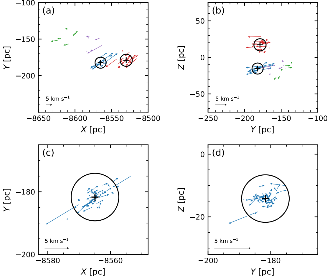
Figure 6. The relative 3D velocity vectors for member candidates projected onto X - Y and Y - Z planes. The red vectors represent the velocities of member candidates of LP 2439 relative to its mean motion, (U, V, W) = (-8.3, 219.1, -4.0) km s -1 , and the blue vectors the velocities of member candidates of NGC 2232 relative to its mean motion, (U, V, W) = (-9.3, 219.2, -3.7) km s -1 are shown in panels (a) and (b). RVs in (a) and (b) are obtained from Gaia DR 2. The center of each cluster is indicated with the (+) symbol. Black circles denote the tidal radii. The purple and green vectors are the relative velocity of member candidates of the purple and green groups, relative to the mean motion of NGC 2232. (c) and (d): The blue vectors represent the relative velocities of members in NGC 2232 that are cross matched with members in Jackson et al. (2020) with membership probability larger than 90%, relative to its mean motion, (U, V, W) = (-9.7, 218.9, -3.8) km s -1 . RVs in (c) and (d) are taken from Jackson et al. (2020). The scale of the velocity vectors is indicated in the bottom-left corner of each panel.
