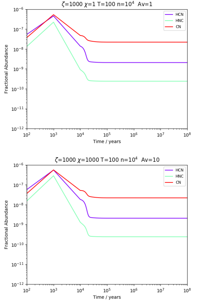
Figure 3. Plots showing the fractional abundances with respect to the total number of hydrogen nuclei of the main isotopologues of the models of Fig. 1.
