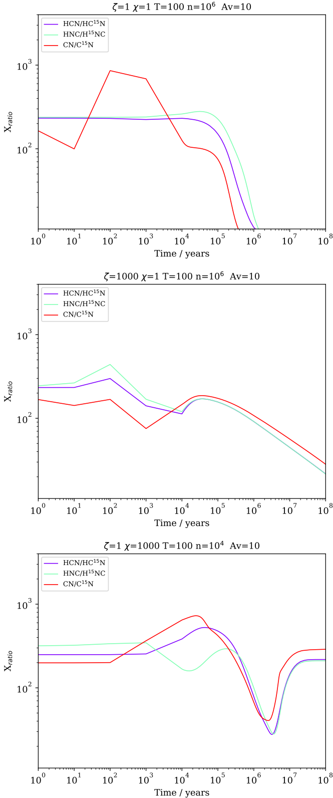
Figure 2. Plots showing the cases with significant ^{14}\text{N}/^{15}\text{N} decrease, i.e. a fractionation increase. Units as in Figure 1.
