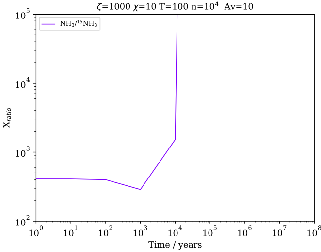
Figure 6. \text{NH}_3 fractionation for one of the best fit model for NGC 253 as derived from the \text{N}_2\text{H}^+ observations.
