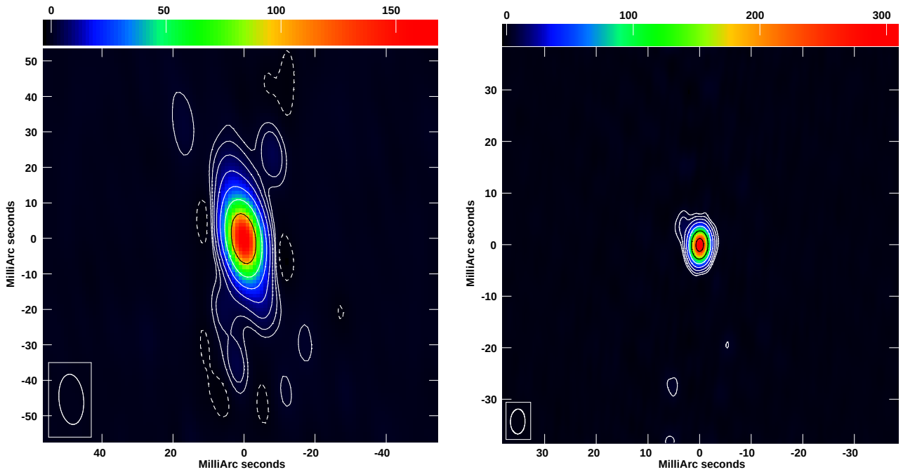
Fig. A.2. Images of the phase reference source J1555–0326 at 1.7 \text{ GHz} ( left ) and 5 \text{ GHz} ( right ). Contour levels are -1, 1, 2, 4, 8, 16, 32, 64 \times the 5\sigma noise level ( 0.3 and 0.8 \text{ mJy beam}^{-1} , for the 1.7 and 5 \text{ GHz} maps, respectively).
