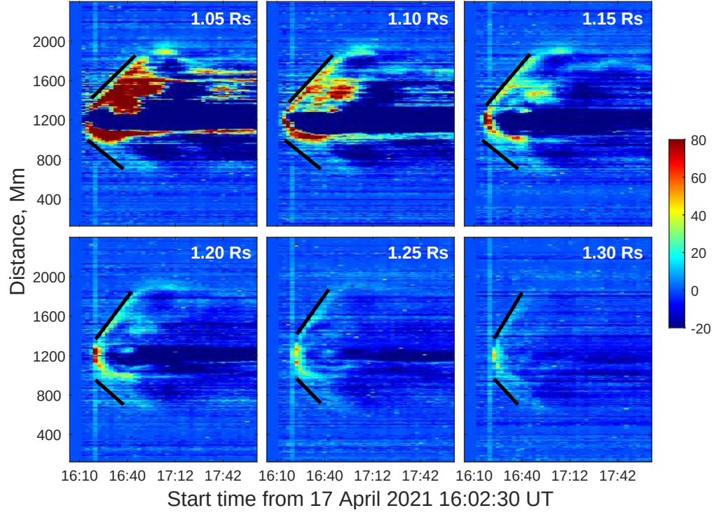
Fig. C.2. Stack plots derived from STEREO A/EUVI 195 Å base-difference images in vertical slits at heights from 1.05 to 1.30 R_{\odot} above the solar surface from the Sun center. The EUV wave fronts are shown by black lines.
