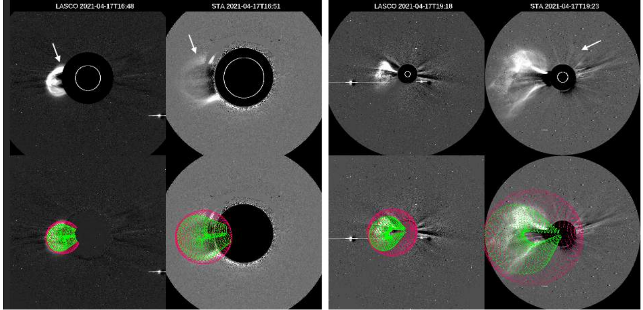
Fig. 7. Base-difference images of the coronagraph observations by SOHO/LASCO/C2 and STEREO A/COR1 (left) and LASCO/C3 and STEREO A/COR2 (right) at different times. The green (red) mesh corresponding to the 3D reconstruction of the CME (CME-driven shock) is shown in the lower panels. The white arrows indicate the signatures of the CME-driven shock.
