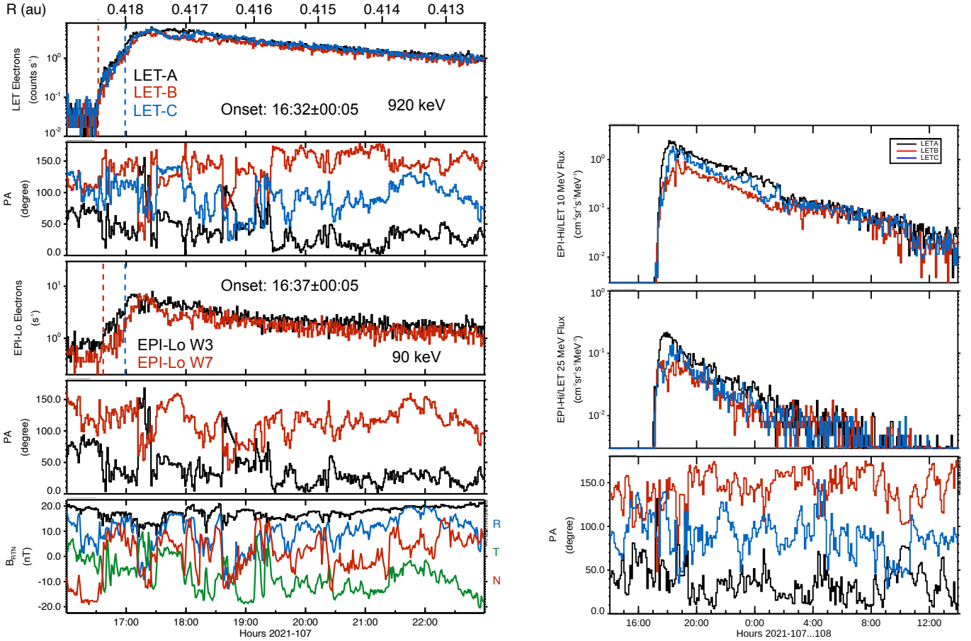
Fig. 16. PSP/IS☉IS observations of the onset of the energetic electron (left) and proton enhancement (right). Top left: Time profile of ~920 keV electrons observed by the three orthogonal EPI-Hi/LET telescope apertures. Left second panel: Pitch angle of each of the EPI-Hi/LET apertures. Left middle: Time profile of ~90 keV electrons observed by EPI-Lo wedges 3 and 7 (sunward and anti-sunward facing, respectively). Left fourth panel: Pitch angle of the boresight of EPI-Lo wedges 3 and 7. Left bottom: Magnetic field magnitude and vector in RTN coordinates as measured by the PSP/FIELDS magnetometer. Top right: Time profile of ~10 MeV protons observed by the three orthogonal EPI-Hi/LET telescope apertures. Right middle: time profile of ~25 MeV protons observed by the three orthogonal EPI-Hi/LET telescope apertures. Right bottom: Pitch angle of each of the EPI-Hi/LET apertures.
